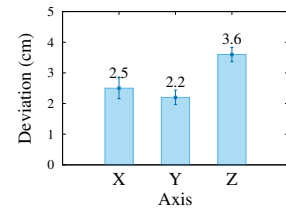
Fig. 7. Coordinates deviation between our ARTag-based sensing and Vicor system.
