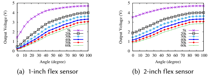
Fig. 4. The change of output voltage as the sensor is being bent with different reference resistors.
