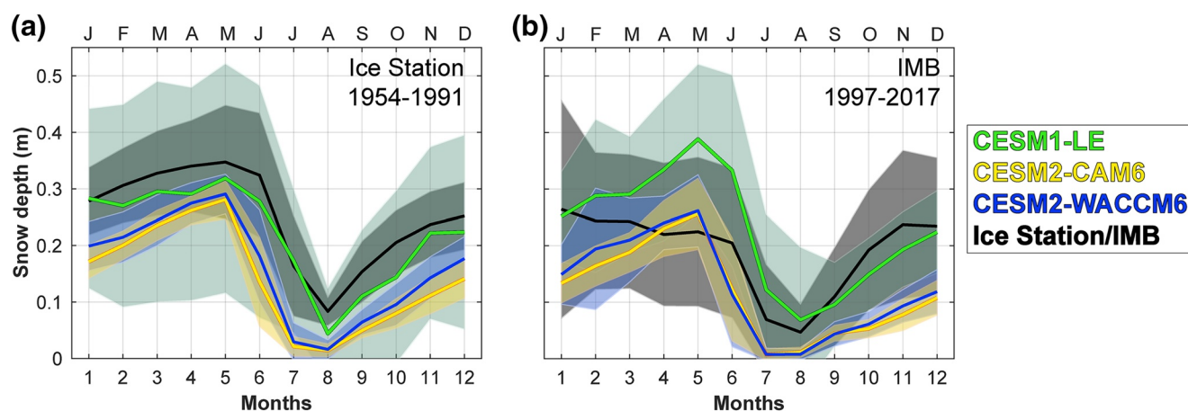
Figure 4. The mean (solid) and standard deviation (shaded spread) in snow depth for the (a) drifting ice stations and CESM configurations, and (b) IMBs and CESM configurations for each month at all drifting IMB/ice station locations. The squared correlation coefficients with the ice stations were 0.15, 0.50, and 0.53 for CESM1-LE, CESM2-CAM6, and CESM2-WACCM6, respectively. The squared correlation coefficients with the IMBs were 0.09, 0.12, and 0.12 for CESM1-LE, CESM2-CAM6, and CESM2-WACCM6, respectively.
