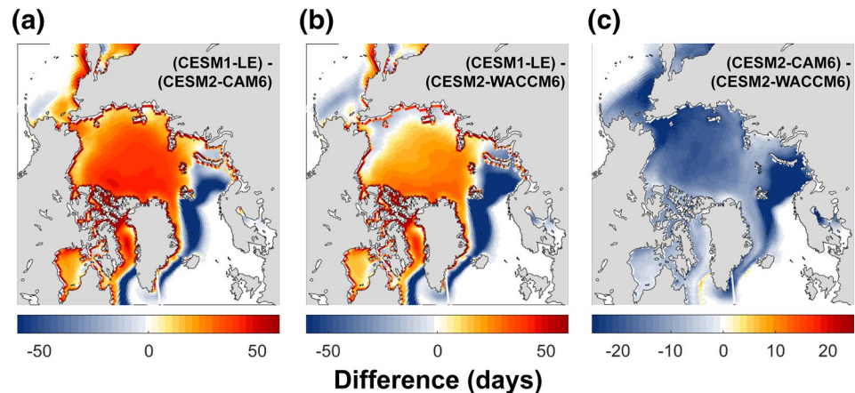
Figure 8. The difference in the snow cover duration, defined as the number of days when the snow cover was at least 0.01 m thick and sea ice concentration at least 15%, over 1920–2100 for (a) CESM1-LE minus CESM2-CAM6, (b) CESM1-LE minus CESM2-WACCM6, and (c) CESM2-CAM6 minus CESM2-WACCM6.
