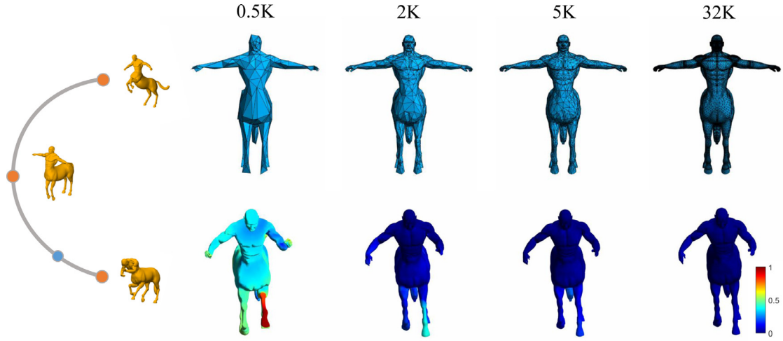
Fig. 7. An example of shape sequence completion from 3 poses of a centaur shape, colored in orange on the left side, using different resolutions of ghost mesh. The top row shows the ghost mesh with different resolutions and the bottom row shows the interpolation error with respect to the one without using ghost. (For interpretation of the references to color in this figure legend, the reader is referred to the web version of this article.)
