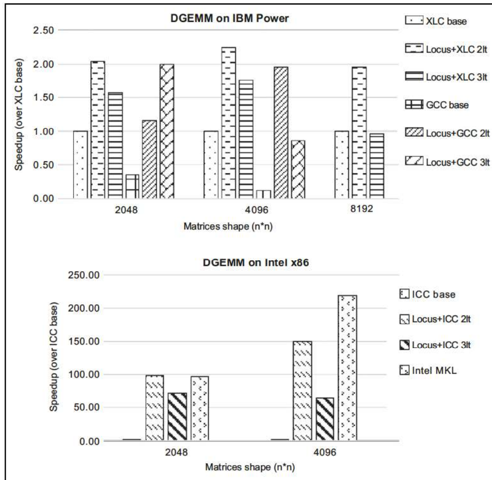
Figure 8. Results for matrix-matrix multiplication on IBM Power 9 and Intel x86. It shows results for the baseline version and the best variant generated by Locus compiled with XLC and GCC. 2t refers to two-level hierarchical tiling and 3t to three-level hierarchical tiling.
