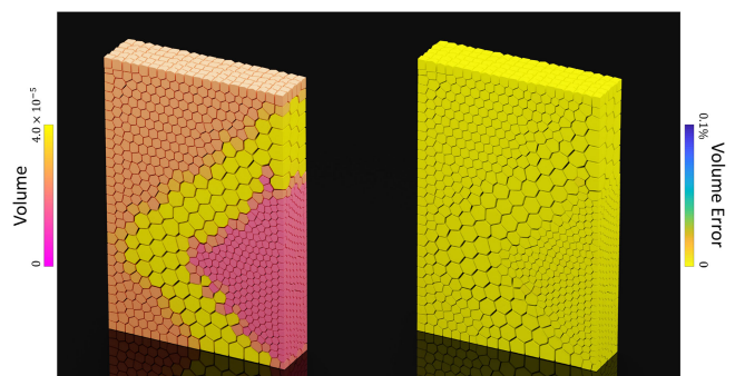
Fig. 16. The 1000-th timestep of a hydrostatic test with various cell volumes. The volume of each cell is shown on the left, and the percentage error, with respect to the initial volume, is demonstrated on the right.
