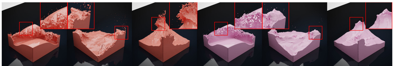
Fig. 12. The rendered results of the double dam break scenario with 1 million staggered Power Particles. The left sequence is simulated with our standard method and the right one with the pressure projection proposed in Sin et al. [35]. Noticeably, our method demonstrates less numerical damping in this comparison.
