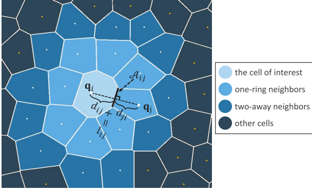
Fig. 1. Exemplary power diagram in 2D.
