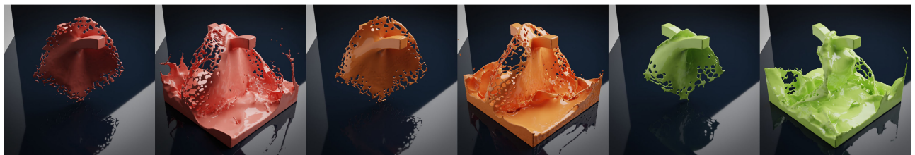
Fig. 10. The rendered results of the colliding fountains scenario. From left to right: 320k staggered Power Particles, 165k adaptive staggered Power Particles, 320k Power Particles. In this test, the 320k staggered Power Particles and 165k adaptive staggered Power Particles are respectively 8 and 15.5 times faster than the 320k Power Particles.
