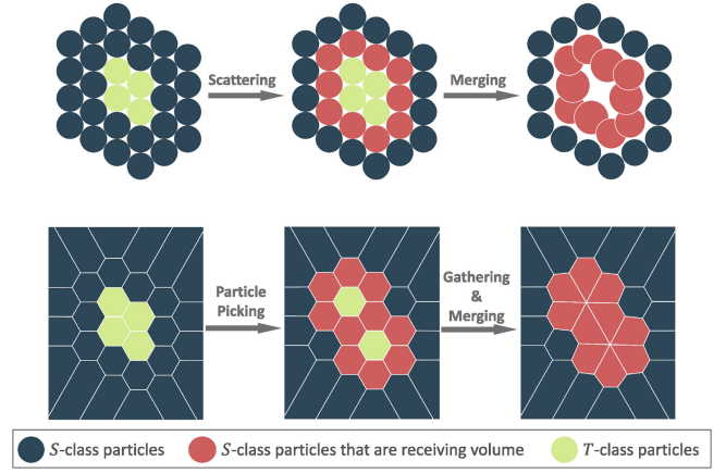
Fig. 7. Previous merging strategy should use atomic scattering operations and would contradict the data dependencies if the merging is applied at once, while ours uses gathering instead and is thread-safe.
