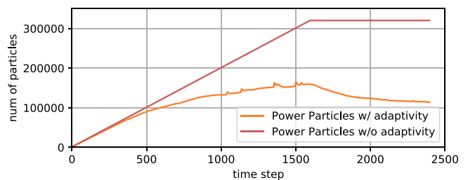
Fig. 17. The statistics of particle number in the colliding fountains scenario (Fig. 10) with adaptivity enabled and disabled. The adaptive particle sampling allows using about half the particles to achieve the similar surface effect.
