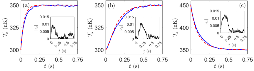
FIG. 1. Rethermalization curves of the pseudotemperatures (a) T_x , (b) T_y , and (c) T_z , with excitation along z , as generated by DSMC simulations (solid blue lines) and solutions to the Enskog equations (dashed red lines). The insets plot the absolute relative error between the DSMC and Enskog solutions to T_j , showing errors on the order of or below 10^{-2} . Simulation parameters are those given in Table I, with the scattering length set to a = 39.8a_0 and \Theta = 90^\circ .
