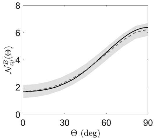
FIG. 2. The number of collisions per rethermalization \mathcal{N}_{zy}^B as a function of \Theta = 0^\circ – 90^\circ , obtained from the theory [Eq. (14); solid black curve] and fits to T_y from DSMC simulations using Eq. (13) (dashed gray curve) with error bars (gray shaded region). These results are found with the parameters in Table I, and a = 39.8a_0 .
