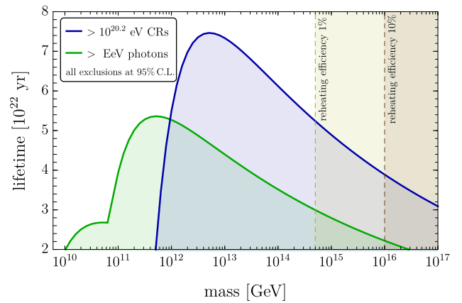
Fig. 1. Constraints on the mass and lifetime of super-heavy DM particles from the absence of UHE photons (green) and from the absence of CR with energy above 10^{20.2} eV (blue). The allowed region lies above the curves. For illustration purpose, the 95% CL upper limit on mass obtained from the possible value of the Hubble rate at the end of inflation for a reheating efficiency of 1% (10%) is shown as the vertical dashed (dotted) line [14].
