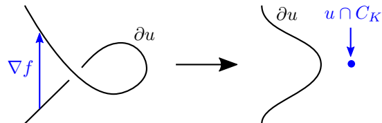
FIGURE 12. From left to right: boundary kink; from right to left: interior kink.
