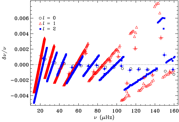
Fig. 11. Relative differences in computed frequencies for the solar-calibrated MESA 1.5 M_\odot , 7 R_\odot model with suitable shifts in mode order (see text), compared with the ASTEC results, in the sense (MESA) – (ASTEC), for l = 0 (black open circles), l = 1 (red open triangles) and l = 2 (blue filled squares). The larger pluses mark the p -dominated modes. The horizontal dotted line indicates zero difference.
