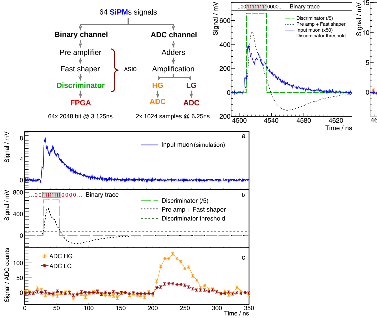
Figure 1: (Top) Schematics of the UMD electronics. (Bottom-a) Simulated SiPM response to a single-muon signal. (Bottom-b) Simulation of the binary mode response to the simulated muon. The discriminator pulse is re-scaled for illustration. (Bottom-c) Simulation of the ADC mode processing. The two ADC outputs (low- and high-gains) are shown.
