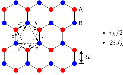
FIG. 1. Yao-Lee model on the honeycomb lattice. The type \lambda of the bond is denoted by x, y, z in the figure. An arrow from site j to i indicates the matrix element h_{ij} of the Hamiltonian of Eq. (3) for u_{ij} = 1 . A solid arrow indicates h_{ij} = 2iJ_\lambda while a dashed line indicates h_{ij} = i\chi/2 .
