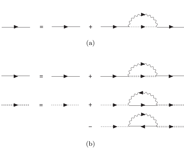
FIG. 3. The Dyson equations for FMs (solid lines) and Majorana fermions (dashed lines). The double lines indicate the full propagators while the single lines are for bare propagators. The wavy lines refer to g^M defined in the text. The diagrams in (a) represent the calculation of \Sigma^{f(1)} in Eq. (8), while the diagrams of (b) are for the calculation of \Sigma^{f(\text{sc})} and \Sigma^{\gamma(\text{sc})} in Eqs. (9) and (11).
