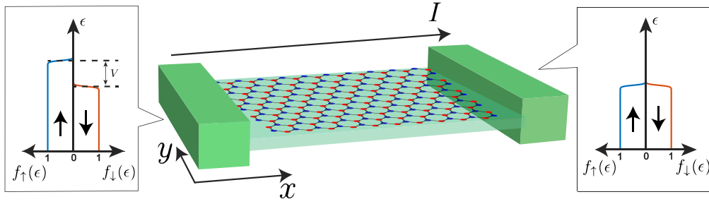
FIG. 2. Schematic of the experiment setup. The spin-up electrons and spin-down electrons in the left spin bath have a chemical potential difference V_s , which drives spin current I_s through the structure.
