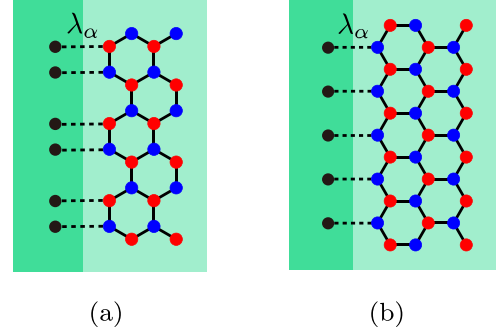
FIG. 4. (a) Armchair-type and (b) zigzag-type contacts. Dashed lines represent the Heisenberg interaction and black dots denote the sites in the spin baths.
