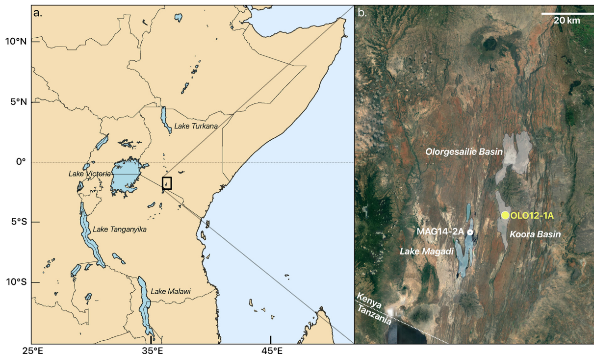
Figure 1. (a) Eastern African study area and (b) regional Google Earth image indicating the Ologesailie Basin, the downstream Kooraa Basin containing OLO12 drill site, and the nearby Lake Magadi with drill core MAG14-2A in the southern Kenya rift.
