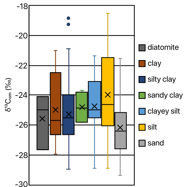
Figure 3. Box and whisker plots of \delta^{13}\text{C}_{\text{OM}} grouped by sediment type in OLO12 demonstrate little effect from lithology on carbon isotope values. The mean is indicated by the ‘x’, upper and lower quartiles with whiskers, middle two quartiles in the box separated by the median (horizontal) line, and outliers as dots.
