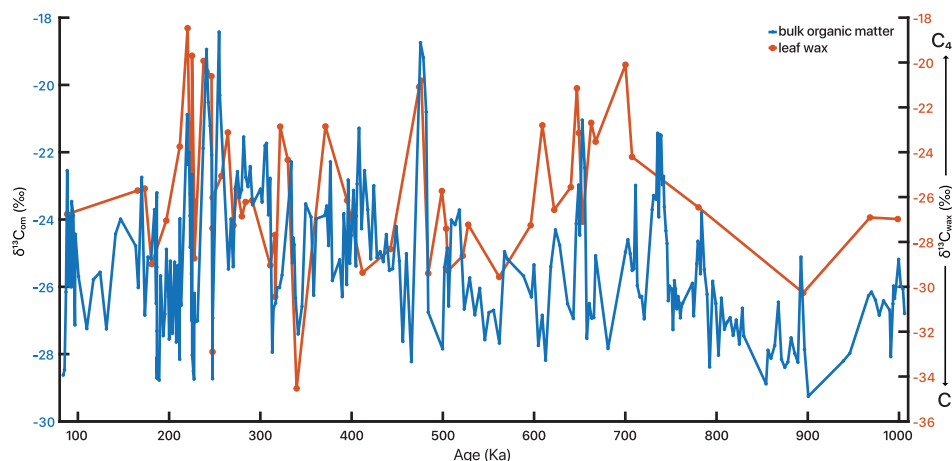
Figure 2. Bulk organic matter carbon isotope record ( \delta^{13}\text{C}_{\text{OM}} ) in blue (y-axis on the left) and plant wax carbon isotope record ( \delta^{13}\text{C}_{\text{wax}} ) in orange (y-axis on the right). The two organic carbon isotope records demonstrate general covariation as well as high-amplitude fluctuations in landscape and environment over the last 1 Myr. (For interpretation of the references to color in this figure legend, the reader is referred to the Web version of this article.)
