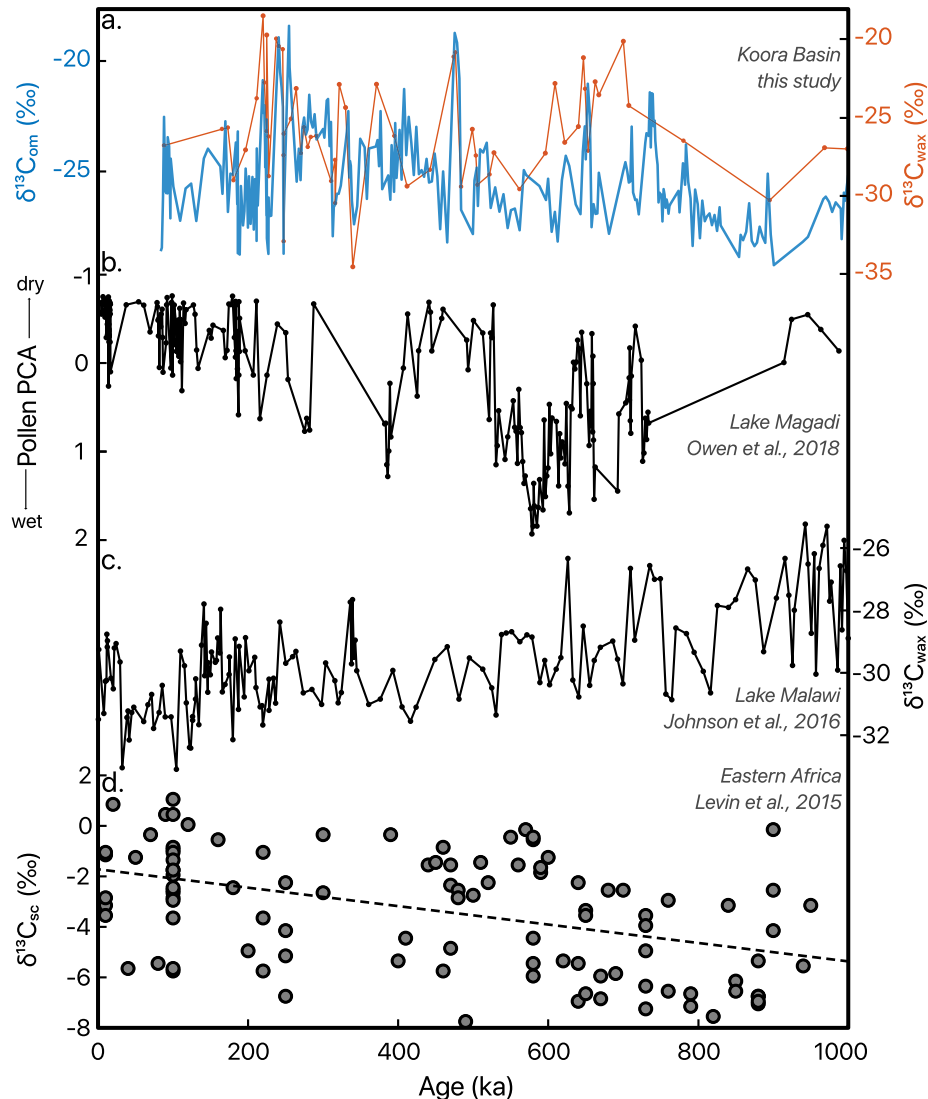
Figure 5. Carbon isotope and pollen records from eastern Africa that span the last 1 Myr demonstrate long-term changes in trend and variance. (a) The \delta^{13}C_{OM} (left, blue) and \delta^{13}C_{wax} (right, orange) from this study compared with the (b) wet/dry first principal component from Lake Magadi (MAG14-2A) pollen (Owen et al., 2018); (c) \delta^{13}C_{wax} from Lake Malawi (Johnson et al., 2016) and (d) \delta^{13}C_{sc} across multiple eastern African basins, which documents a gradual C_4 expansion, denoted by linear regression (Levin, 2015 and references therein). PCA = principal component analysis. (For interpretation of the references to color in this figure legend, the reader is referred to the Web version of this article.)
