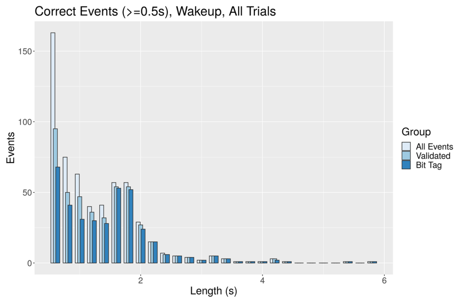
Fig. 9 Histogram of correctly identified events, by event length
