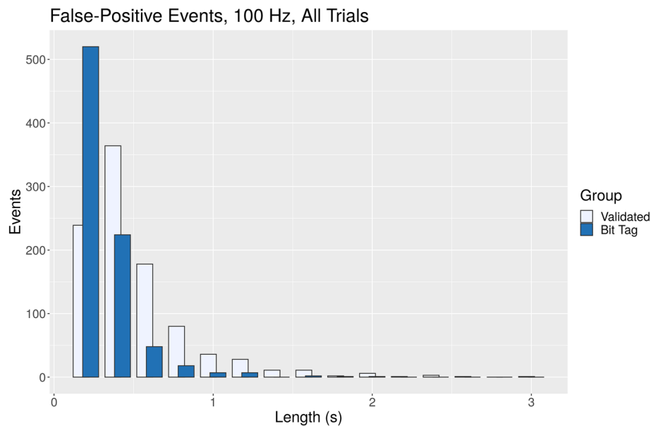
Fig. 8 False-positive events in each simulation, arranged by length. False-positives events are those that contain no samples marked as part of a motion event by video analysis. The majority of such false-positive events are very brief, lasting no longer than 1 s. The bars are “overlapped” to show differences in counts between the groups
