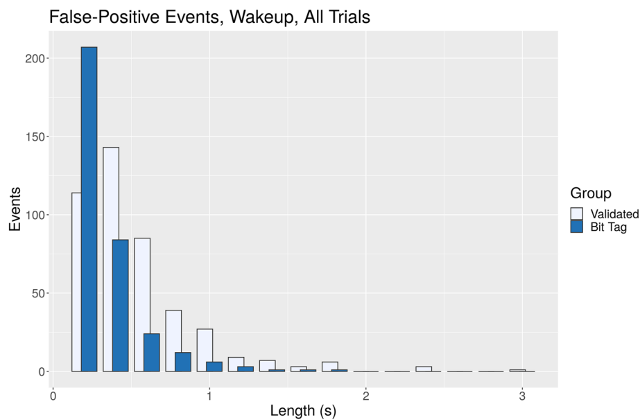
Fig. 10 False-positive events in simulations using wakeup mode
