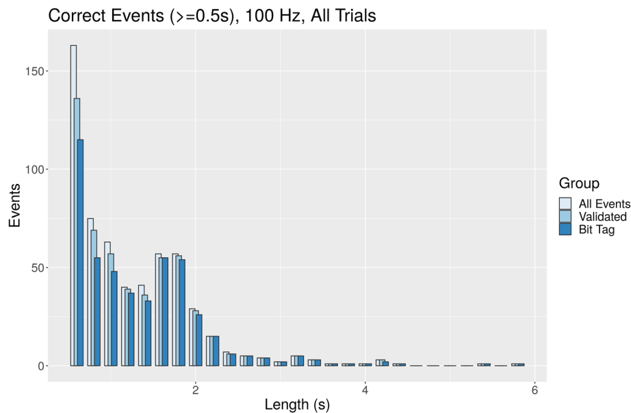
Fig. 7 Histogram of correctly identified events, by event length, without using the Wakeup mode. “All Events” represents the total number of motion events of a particular length that were identified during video analysis. “Validated” corresponds to events detected by the simulated activity detector when configured with parameters found using our validation methodology. “Bit Tag” corresponds to the performance of the activity detector using parameters determined prior to the development of our current methodology. The histogram bars are “overlapped” to show differences in event counts between methods
