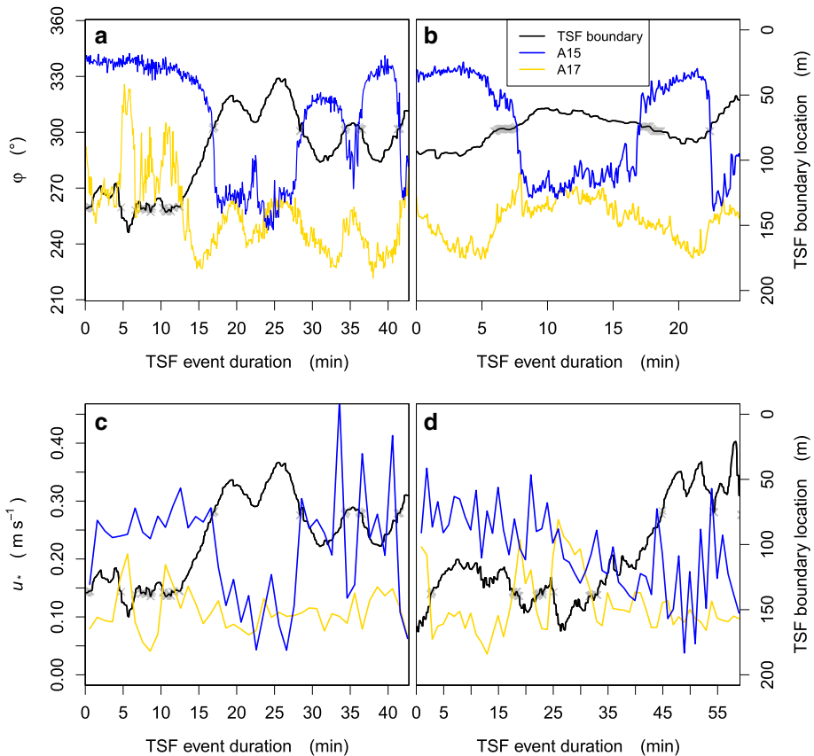
Fig. 14 a, b Time series of wind direction \varphi at two ultrasonic anemometer stations. c, d Time series of friction velocity u_* at the same stations. Grey crosses: A15 (at 75 m) or A17 (at 138 m) within the transition area of TSFs; black line: location of TSF boundary
