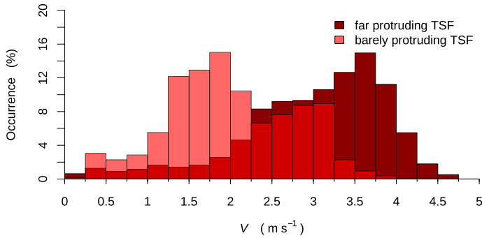
Fig. 13 Histogram of mean wind speed V for station A9 on the north shoulder plotted for a far (red) and a barely (pink) protruding TSF. Colours are opaque to show the overlapping histograms simultaneously
