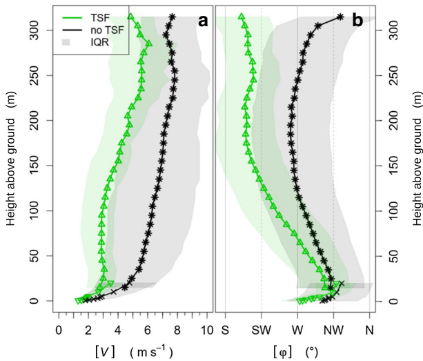
Fig. 7 Conditional averaging of a wind speed [V] and b wind direction [\varphi] during the occurrence (green) and absence of TSFs (black). Inverted triangles and crosses: 20-m tower; triangles and stars: wind profiler; shaded areas: inter-quartile range (IQR) of [V] and standard deviation of [\varphi]
