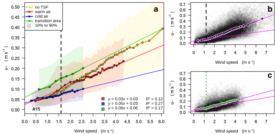
Fig. 11 The relation of wind speed to friction velocity u_* following Sun et al. (2012). Vertical lines show the wind-speed threshold separating the weak-wind from the strong-wind regime for a all night-time data, b weak static stability during the absence of TSFs, and c elevated static stability during the occurrence of TSFs. Further, equally sized bin averages are added (lines with dots) as well as the linear correlation lines for a the air layer of the TSFs or b , c each wind regime. a Each air layer of the TSF is coloured differently and the polygons show the range of the 10–90% percentile of u_*
