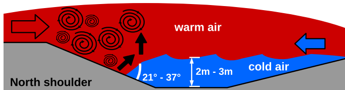
Fig. 1 Conceptual drawing (cf. Pfister et al. 2021) of a TSF (not to scale) within the valley (grey areas) consisting of a warm-air layer (red) and a cold-air layer (blue). Coloured arrows indicate the different flow direction of the air layers, while black swirls indicate the topographically-induced mixing. At the transition area, where the air layers merge, the warm-air layer is pushed upwards (black arrow) as the cold-air layer acts as a barrier
