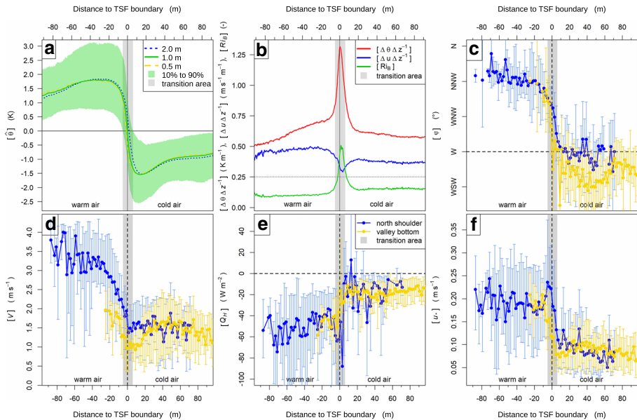
Fig. 3 Most important parameter describing TSFs (1-min averages) which are conditionally averaged depending on their distance to the boundary of the fronts from Part 1 (Pfister et al. 2021). Fibre-optic measurements of a spatial temperature perturbation [\theta] and b the bulk Richardson number [Ri_B] derived from the ratio of the buoyancy gradient [\Delta\theta \Delta z^{-1}] to the wind shear [\Delta u \Delta z^{-1}] as well as ultrasonic anemometer measurements showing c the mean wind direction [\varphi] , d mean wind speed [V] , e sensible heat flux [Q_H] and, f friction velocity [u_*]
