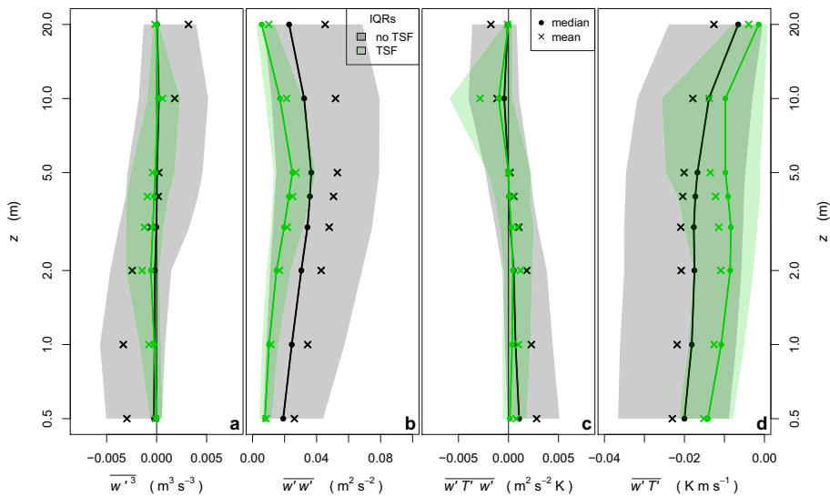
Fig. 4 Profiles of the third-order moment of the a vertical velocity component \overline{w'^3} and c sensible heat flux \overline{w'T'w'} on the main tower and the corresponding profiles of the second-order moments b \overline{w'w'} and d \overline{w'T'} during the occurrence and absence of TSFs. Areas: inter-quartile range (IQR)
