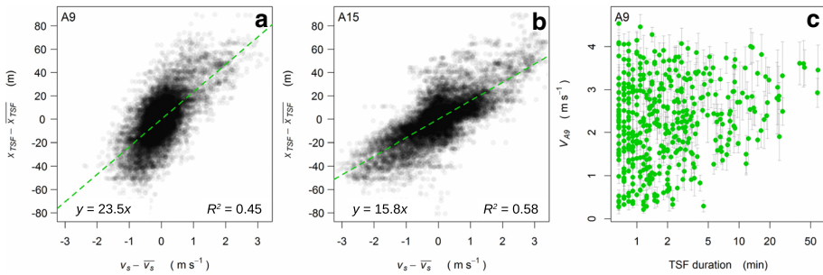
Fig. 6 Variation of the north–south component of the velocity v_s - \bar{v}_s plotted against the variation of the TSF boundary location x_{TSF} - \bar{x}_{TSF} determined during each TSF event for, a station A9 on north shoulder, and b station A15 half-way uphill on the north shoulder. c Duration of TSF events plotted against the mean wind speed at A9
