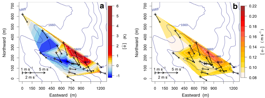
Fig. 5 Overview of field site with elevation shown by contour lines (dark blue). a The mean spatial temperature perturbation, [\hat{\theta}] , and b the mean friction velocity, [u_*] , during the occurrence of TSFs is added by filled contour lines (see colour scale). Black arrows show flow direction and strength
