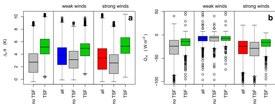
Fig. 9 Boxplots of a static stability \Delta_z\theta and b sensible heat flux Q_H for the 1-m station on the main tower. The boxplots are classified by the occurrence of TSFs as well as wind regimes introduced by Sun et al. (2012) (cf. x-axis)
