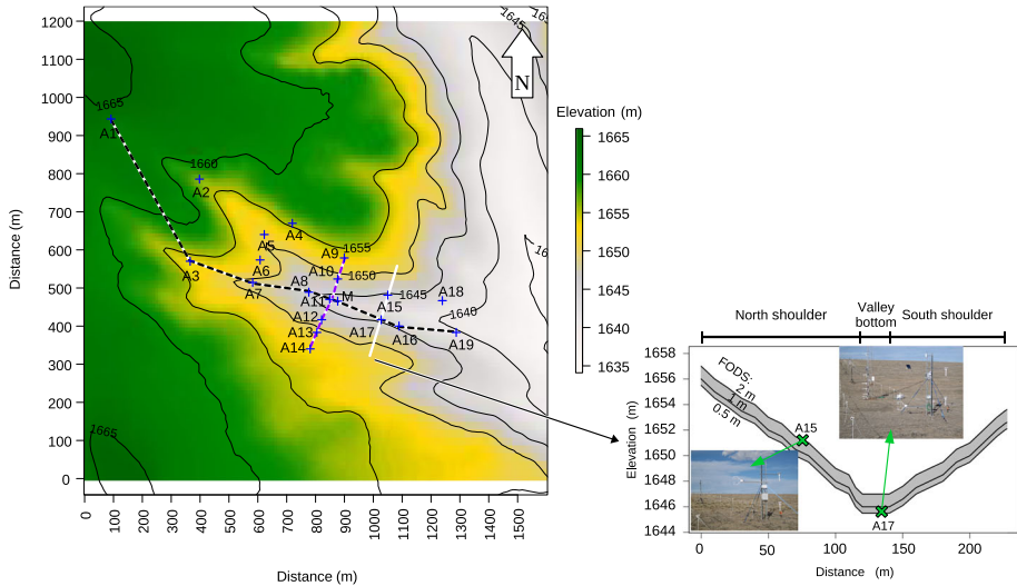
Fig. 2 Left: Topographical overview of field site with ultrasonic anemometer stations (A1–A19), the 20-m main tower (M), and the FODS transect (white line). Right: Cross-valley view of the fiber-optic transect showing its length and elevation (after Pfister et al. 2021)
