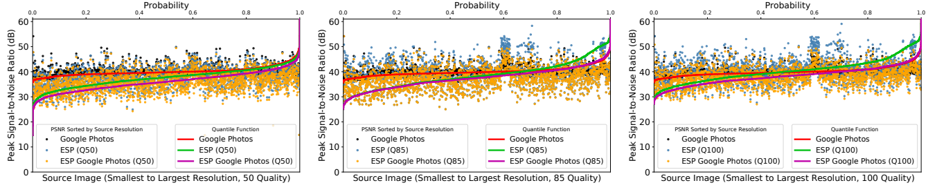
Figure 5: Image quality measured using PSNR relative to source images.
