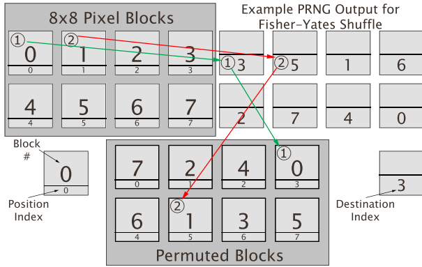
Figure 3: Example of 8×8 block permutation.
