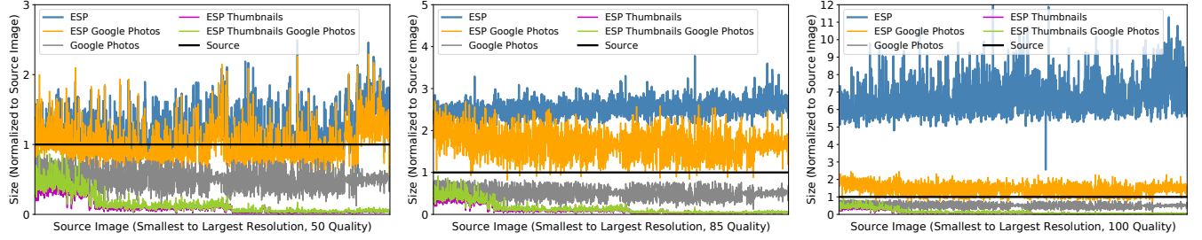
Figure 6: Image file size overhead normalized against source images.
