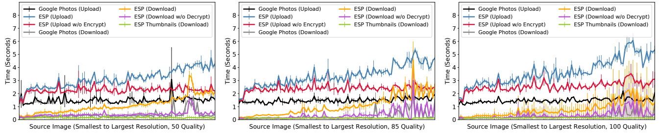
Figure 7: Image upload and download times using Google Photos.
