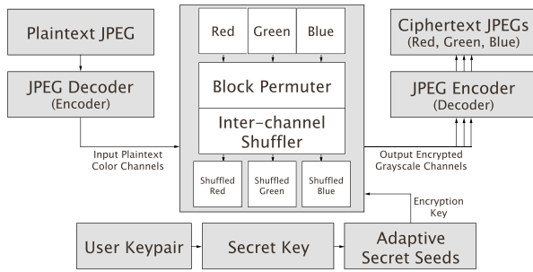
Figure 1: The ESP encryption architecture for JPEGs.
