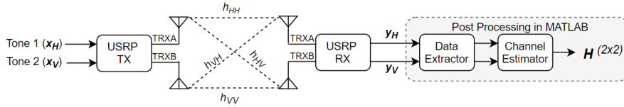
Fig. 3: 2x2 Channel Sounding System Model.
