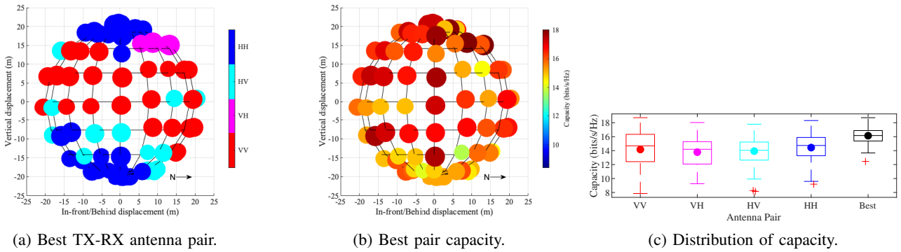
Fig. 6: Best performing TX-RX antenna pair (a) and its capacity (b). Distribution of measured capacity over 3D space of four fixed TX-RX pairs and "best-pair" selection strategy (c.)
