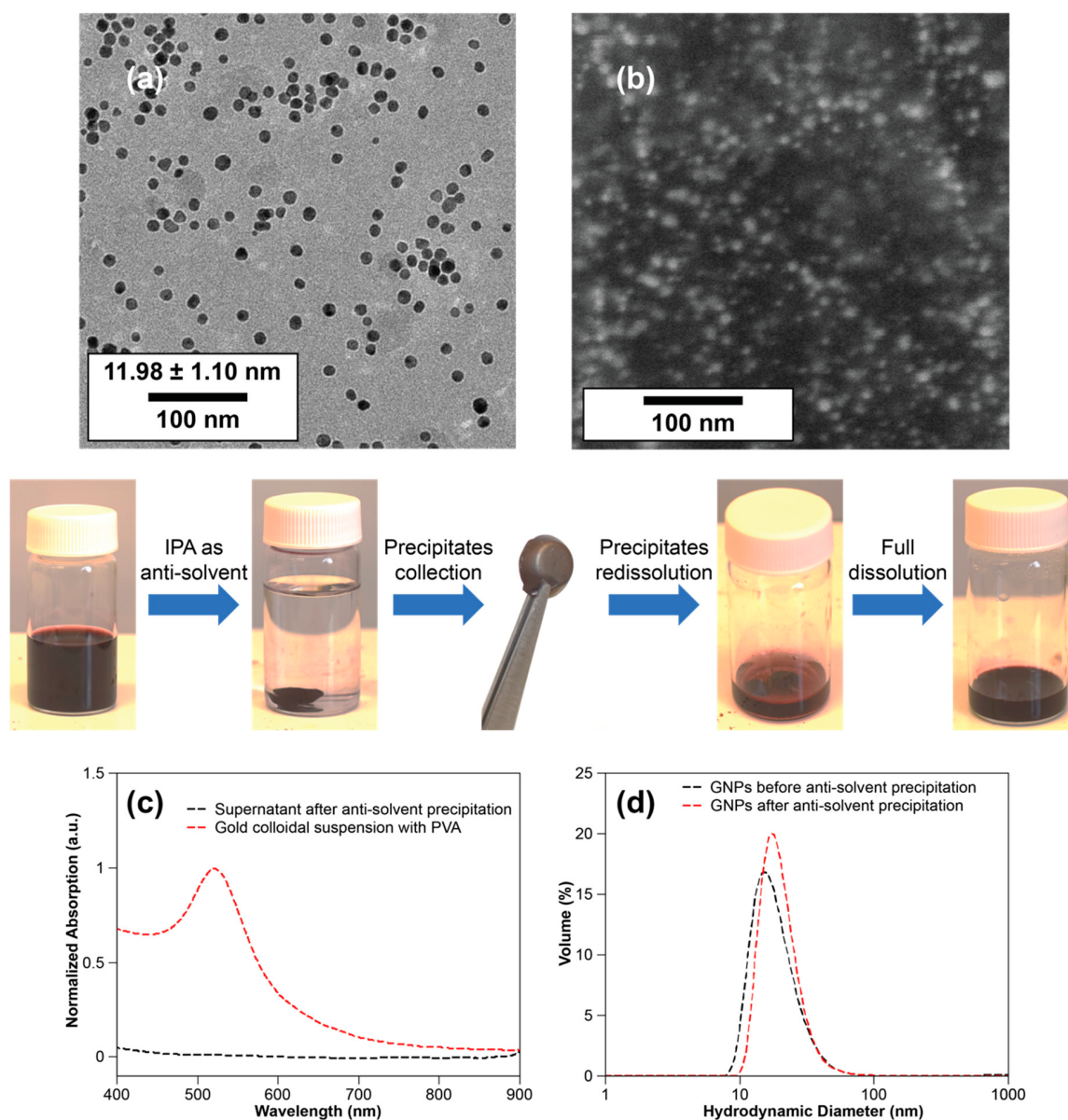
Figure 8. Diagram of anti-solvent precipitation and the re-dissolution process (mid-row); (a) TEM image of GNPs (10 mM gold ions, Ct/Au \equiv 3); (b) SEM image of Au/PVA nanocomposite obtained from anti-solvent precipitation; (c) UV-vis absorption of the gold colloidal suspension with PVA and supernatant after anti-solvent precipitation; (d) size distributions of GNPs before and after anti-solvent precipitation from DLS.
