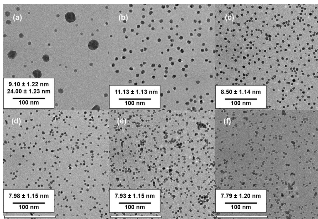
Figure 4. TEM images of GNPs (5 mM gold ions, 0.5% PVA) with variable of Ct/Au and size distribution analyzed using Image J. (a) TEM image of GNPs with Ct/Au = 1; (b) TEM image of GNPs with Ct/Au = 3; (c) TEM image of GNPs with Ct/Au = 6; (d) TEM image of GNPs with Ct/Au = 9; (e) TEM image of GNPs with Ct/Au = 12; (f) TEM image of GNPs with Ct/Au = 15.
