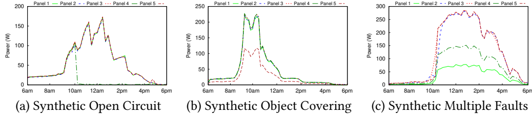
Fig. 10. Synthetic fault injection with (a) open circuit fault, (b) leaves covering fault, (c) multiple leaves covering faults
