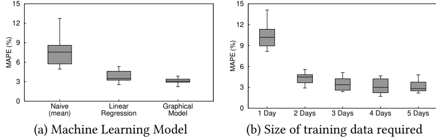
Fig. 8. Prediction model accuracy and the size of training data required.
