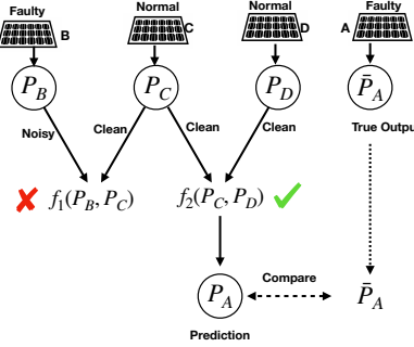
Fig. 3. A forecasting model is used to ensure non-noisy inputs to our Bayesian model.
