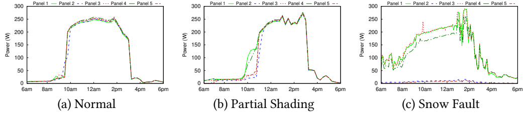
Fig. 4. Residential home power output on an example day under (a) normal condition, (b) partial shading on some panels on east side, (c) snow covering on some of the panels.
