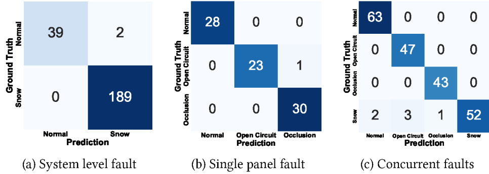
Fig. 12. Classification accuracy for (a) system-wide snow faults, (b) single panel faults, (c) multiple panel faults.
