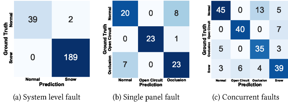
Fig. 11. Classification accuracy for our baseline linear regression anomaly detection method for (a) system-level faults, (b) single panel faults, (c) multiple panel faults.
