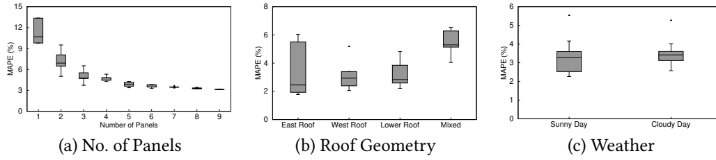
Fig. 9. Effect of various factors on the model accuracy (a) number of panels, (b) roof geometry, and (c) weather. evaluate the overall model's performance, while sensitivity and specificity are used to test how accurate the model is to correctly detect the anomalies and normal cases.
