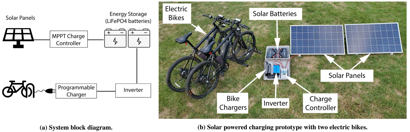
Figure 2: (2a) Block diagram of our solar charging station prototype, and (2b) a photo of our setup with two electric bikes.
