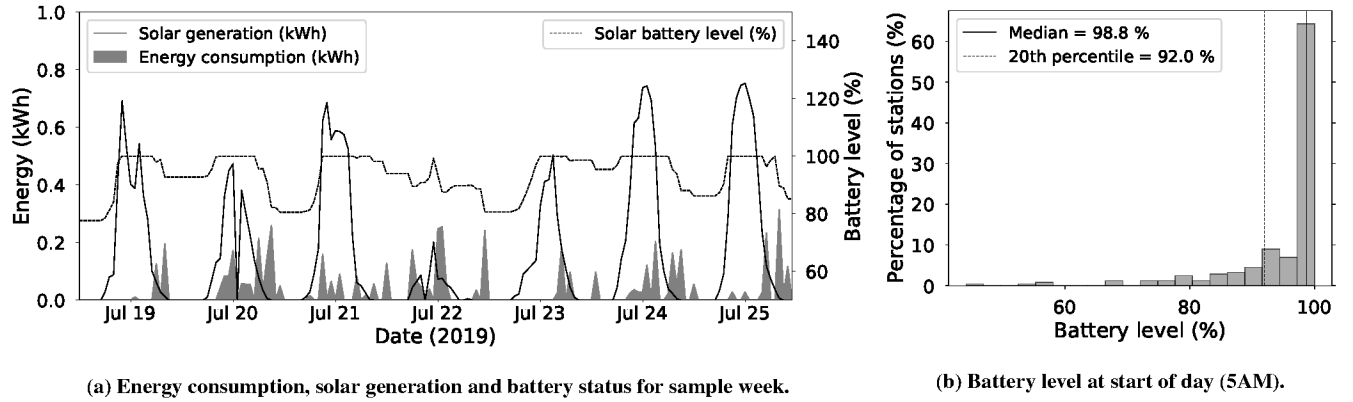
Figure 12: (12a) Energy consumption, solar generation and battery level for sample station during a week, and (12b) solar battery level at start of day before solar generation.
