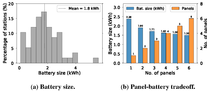
Figure 14: (14a) Battery size by peak energy demand, and (14b) tradeoff between number of panels and required battery size.
