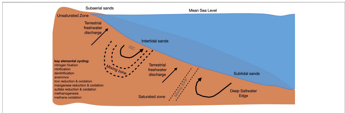
FIGURE 1 | Diagram of a beach aquifer. Adapted from Robinson et al., 2018 and Ruiz-González et al., 2021 (ISC: intertidal saltwater cell).
