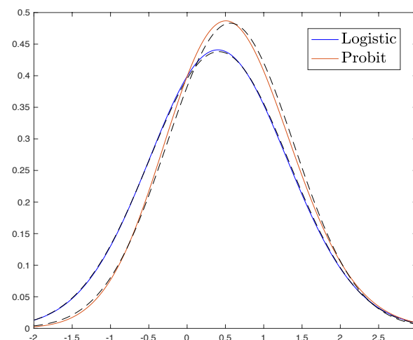
Figure A2. Probability distribution function of SY for the logistic and Probit models ( \|x_0\|_2 = 1 ) compared with the probability distribution function of the Gaussian random variable (dashed lines) with the same mean and variance i.e., \mathcal{N}(\mathbb{E}[SY], \text{Var}[SY]) .
