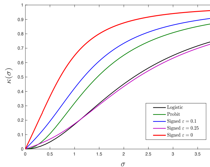
Figure A1. The value of \kappa(\sigma) as in Theorem 2 for various measurement models. Since \kappa(\sigma) is a monotonic function of \sigma , the solution to \kappa(\sigma) = 1/\delta determines the minimum possible value of \sigma .
