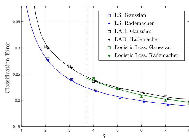
Figure 2. Theoretical (solid lines) and empirical (markers) results of classification risk in GMM as in Theorem 4 and (39) for LS, LAD and logistic loss functions as a function of \delta for r = 1 . The vertical line represents the threshold \delta^* \approx 3.7 as evaluated by (36). Logistic loss gives unbounded solution if and only if \delta < \delta^* .
