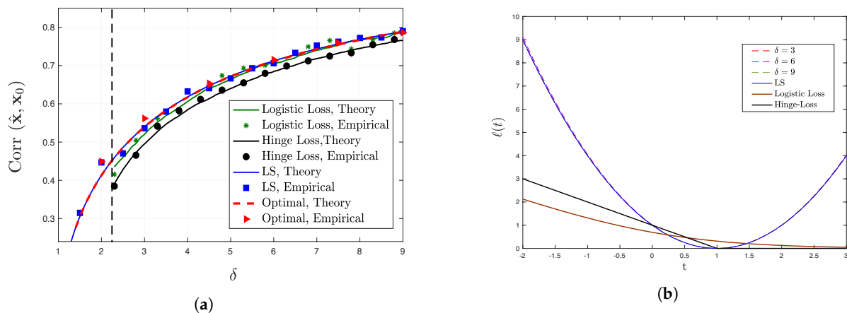
Figure 3. (a) Comparison between analytical and empirical results for the performance of LS, logistic loss, hinge loss and optimal loss function for logistic model. The vertical dashed line represents \delta_f^* \approx 2.275 , as evaluated by (35). (b) Illustrations of optimal loss functions for different values of \delta , derived according to Theorem 3 for logistic model. To signify the similarity of optimal loss function to the LS loss, the optimal loss functions (hardly visible) are scaled such that \ell(1) = 0 and \ell(2) = 1 .
