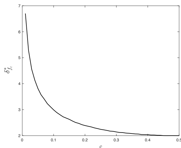
Figure A3. The value of the threshold \delta_{f_\varepsilon}^* in (A69) as a function of probability of error \varepsilon \in [0, 1/2] . For logistic and hinge losses, the set of minimizers in (3) is bounded (as required by Theorem 1) iff \delta > \delta_{f_\varepsilon}^* .
