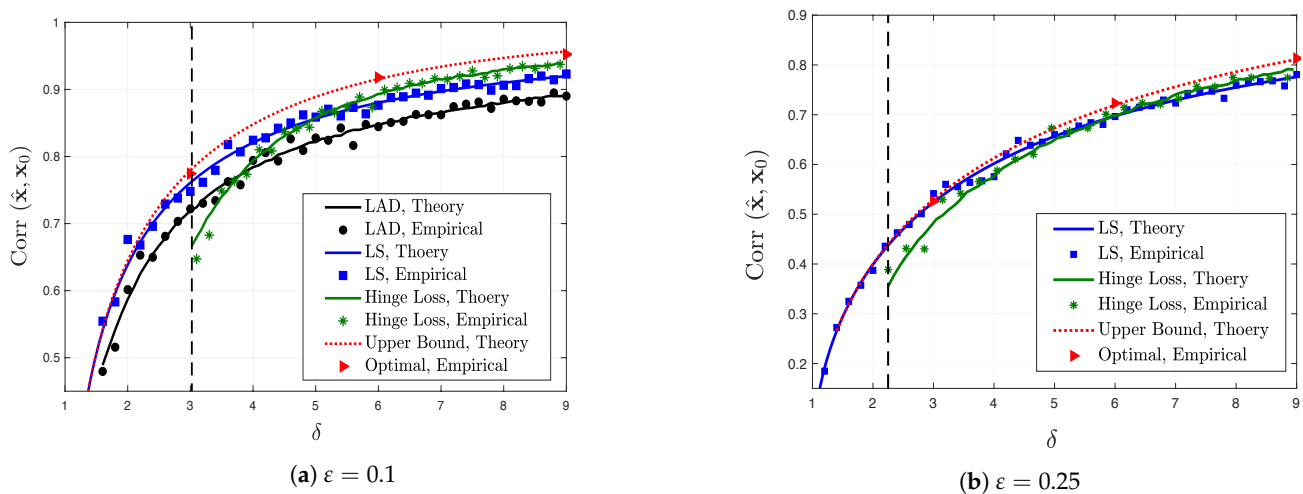
Figure A4. Comparisons between analytical and empirical results for the least-squares (LS), least-absolute deviations and hinge loss functions along with the upper bound on performance and the empirical performance of optimal loss function as in Theorem 3, for noisy-signed measurement model with \varepsilon = 0.1 (a) and \varepsilon = 0.25 (b). The vertical dashed lines are evaluated by (A69) and represent \delta_{f_\varepsilon}^* \approx 3 and 2.25 for \varepsilon = 0.1 and 0.25 , respectively.
