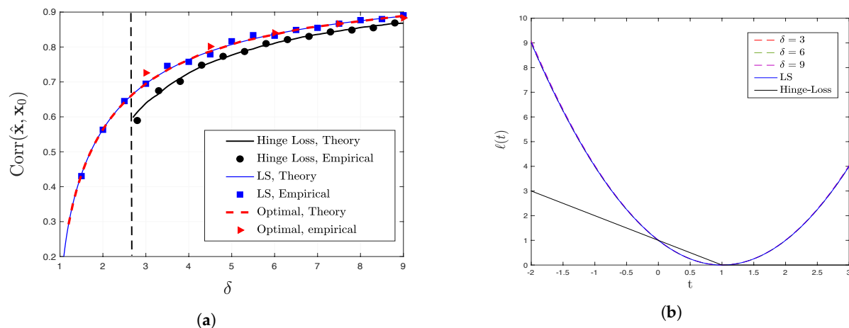
Figure 4. (a) Comparison between analytical and empirical results for the performance of LS, hinge loss and optimal loss function for Probit model. The vertical dashed line represents \delta_f^* \approx 2.699 , as evaluated by (35). (b) Illustrations of optimal loss functions for different values of \delta derived according to Theorem 3 for Probit model. To signify the similarity of optimal loss function to the LS loss, the optimal loss functions (hardly visible) are scaled such that \ell(1) = 0 and \ell(2) = 1 .
