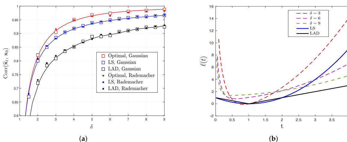
Figure 1. (a) Comparison between theoretical (solid lines) and empirical (markers) performance for least-squares (LS) and least-absolute deviations (LAD), as predicted by Theorem 1, and the optimal performance, as predicted by the upper bound of Theorem 2, for the signed model. The squares and circles denote the empirical performance for Gaussian and Rademacher features, respectively. (b) Illustrations of optimal loss functions for the signed model for different values of \delta according to Theorem 3.
