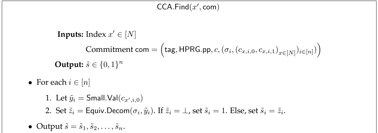
Figure 1: Routine CCA.Find
