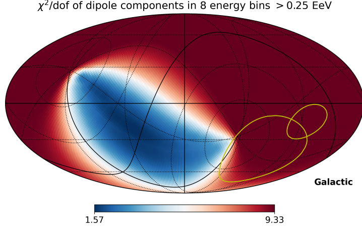
Figure 2: \chi^2/n_{\text{dof}} for the dipole direction of highest energy Galactic CRs; an Equatorial Coordinate grid is overlaid. The dipole pointing toward or away from the Galactic center is excluded by more than 6\sigma . The 1\text{-}\sigma domains of the direction of the total dipole in the 4-8 EeV and >8 EeV bins measured by Auger [12] are the large and small yellow ovals.
