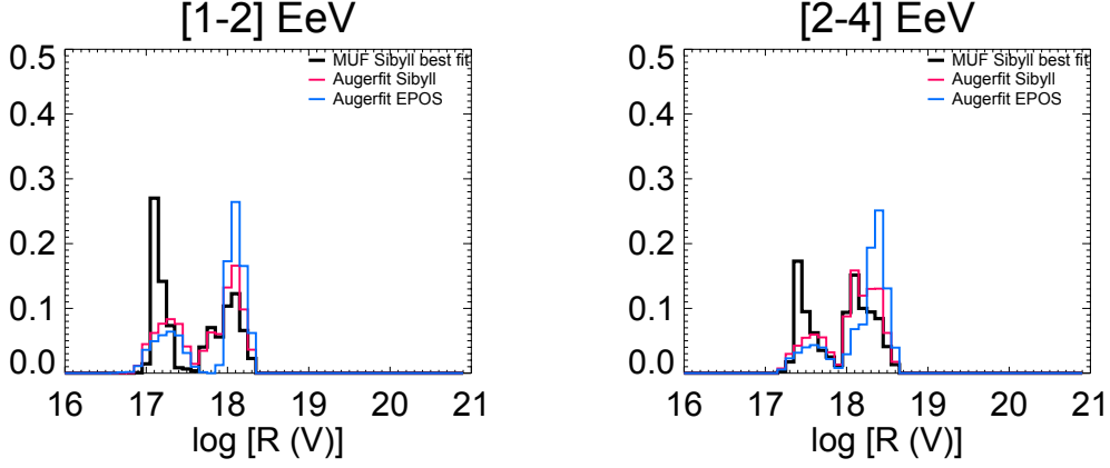
Figure 1: The rigidity breakdown as a function of energy from Auger using 2 different models, and from the modeling of MUF19 (dashed, thin lines and solid, respectively).
