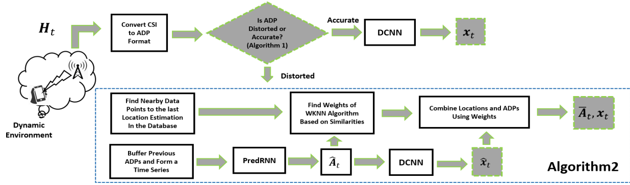
Fig. 3: Block Diagram of the proposed localization framework DyLoc.
