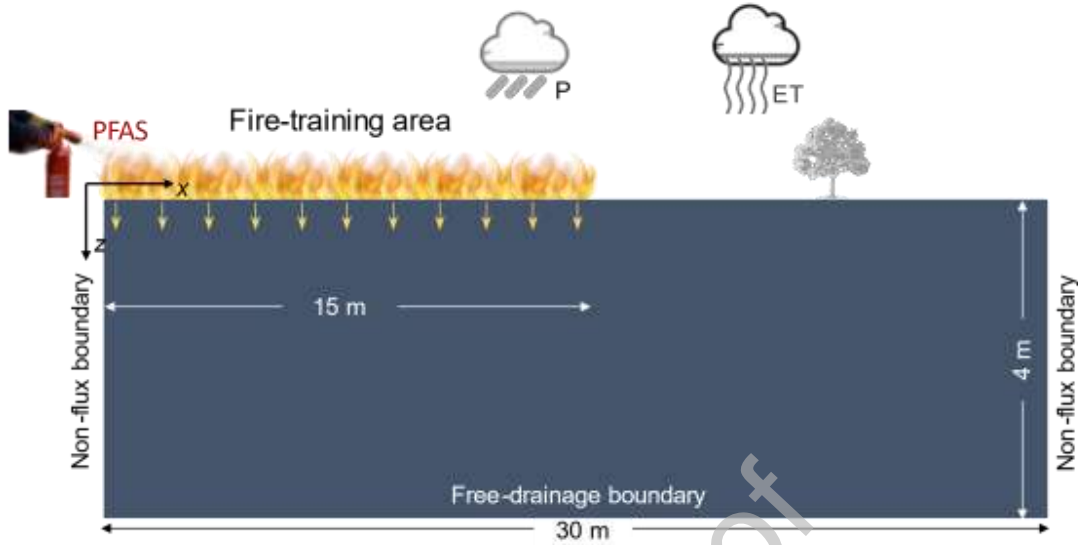
Figure 2 A schematic for PFAS release to a homogeneous vadose zone at a model FTA site ( x - z cross-sectional view). The vadose zone is composed of Accusand, Vinton, or Hayhook. Note that the FTA is assumed symmetric and only half of it is shown.
