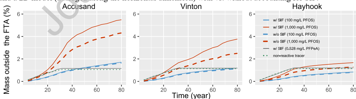
Figure 5 The fraction of PFOS mass spread outside of the vadose zone directly underneath the FTA. The results include different porous media (i.e., Accusand, Vinton, and Hayhook), different release concentrations (100 mg/L vs. 1,000 mg/L for PFOS, 0.528 mg/L for PFPeA, and 0.528 mg/L for the non-reactive tracer), and with vs. without accounting for SIF.
