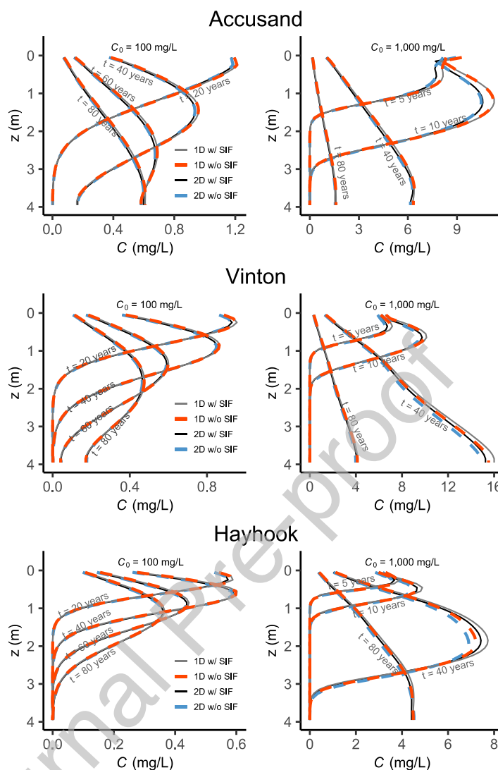
Figure 4 Time-dependent vertical profiles of the aqueous PFOS concentration obtained from a 1D model and a 2D model (averaged along the horizontal dimension) with vs. without accounting for SIF.
