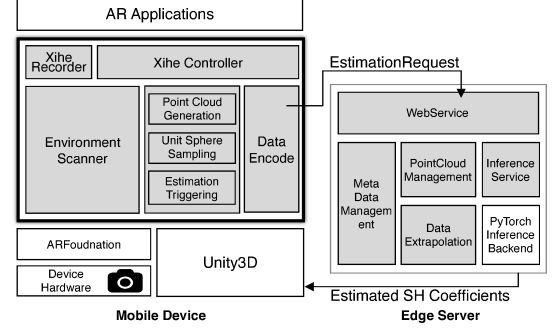
Figure 6: XIHE architecture.
