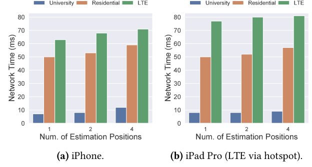
Figure 9: XiHE network time. We measure the time needed to transfer the encoded point cloud of 1280 anchors and to receive the lighting estimation SH coefficients.
