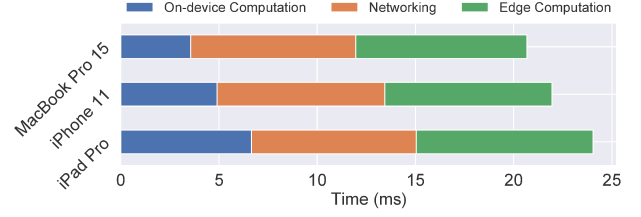
Figure 7: XIHE end-to-end time. XIHE lighting estimation via the university WiFi, can complete in as fast as 20.67ms.
