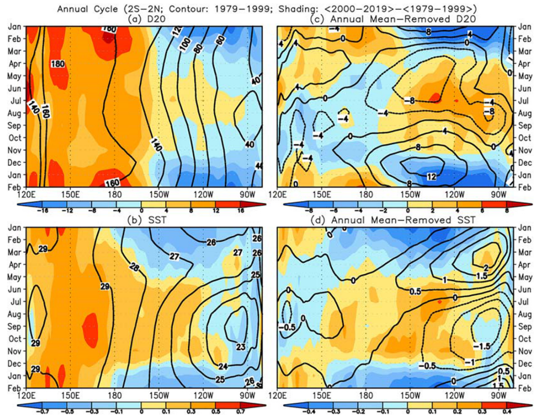
Figure 8. Annual cycle of (a) D20 and (b) SST and annual mean-removed annual cycle of (c) D20 and (d) SST averaged in 2°S–2°N for the mean in January 1979 to December 1999 (contours) and the difference of the mean in January 2000 to December 2019 minus the mean in January 1979 to December 1999 (shading). (c, d) The results with annual mean removal. The units are m for D20 and °C for SST.
