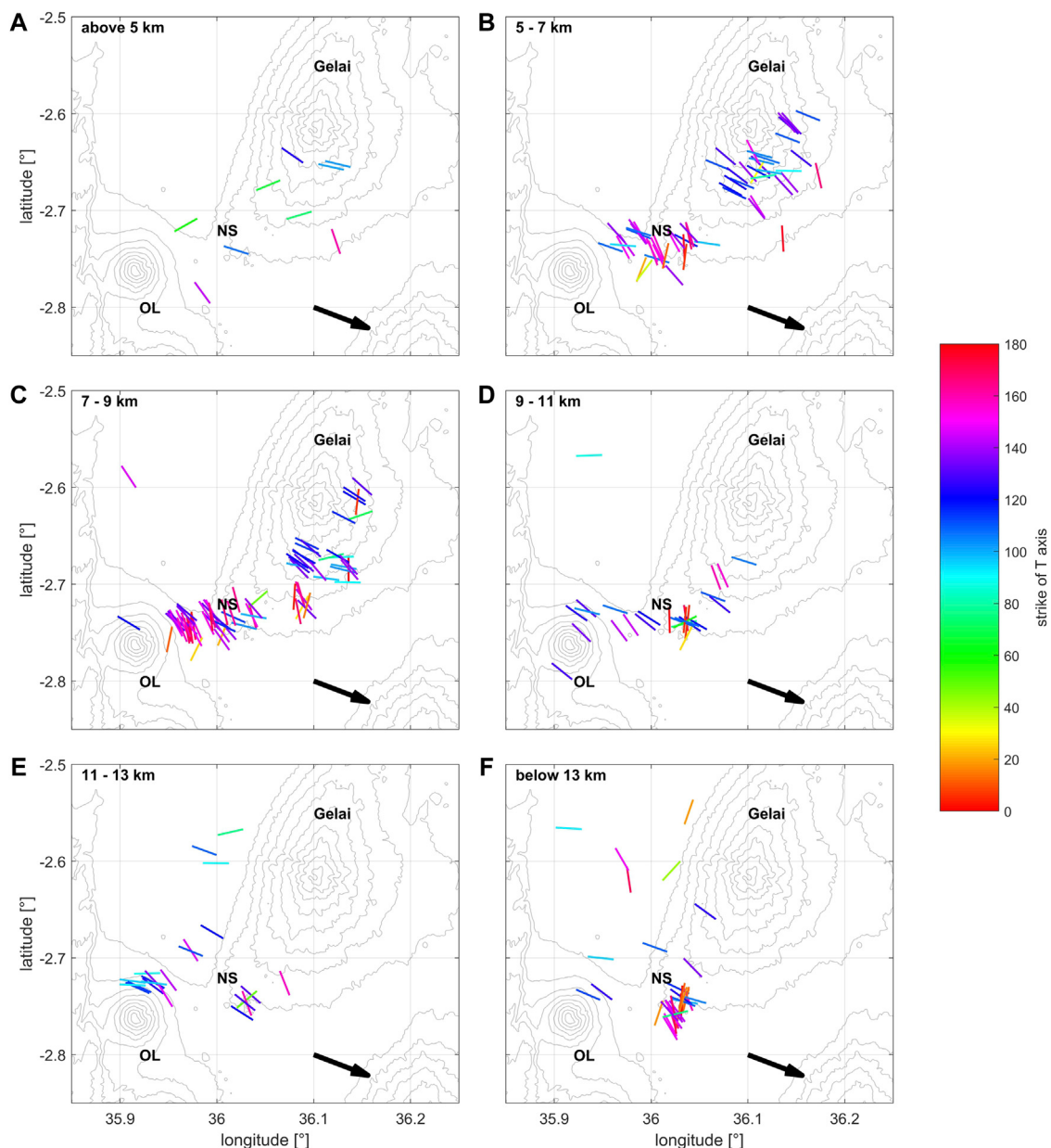
FIGURE 8 | Map view of T-axis direction of focal mechanisms. Axes are centered on earthquake location and colored by their azimuth. (A) 0–5 km depth. (B) 5–7 km depth. (C) 7–9 km depth. (D) 9–11 km depth. (E) 11–13 km depth. (F) below 13 km depth.
