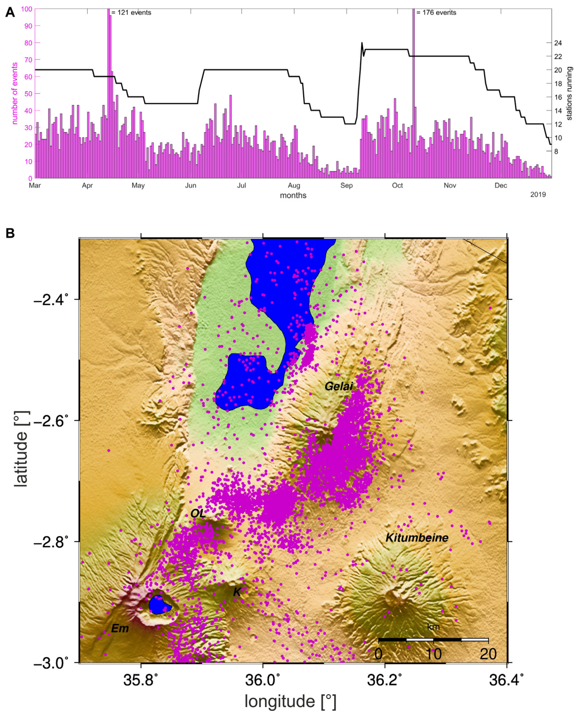
FIGURE 3 | (A) Histogram of well-located earthquakes per day ( left y-axis ) and superimposed numbers of running stations ( right y-axis ). (B) Seismicity map, small circles show earthquakes.
