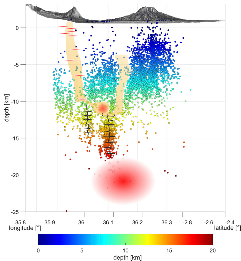
FIGURE 12 | Plumbing system of Oldoinyo Lengai with seismicity. The orange shaded areas are seismic gaps interpreted as part of the mushy plumbing system, overlain with small reddish ellipses denoting sill complexes. Black lines denote deep plumbing system, which connect the hydrothermal system to the deep magma chamber inferred from Roecker et al. (2017).
