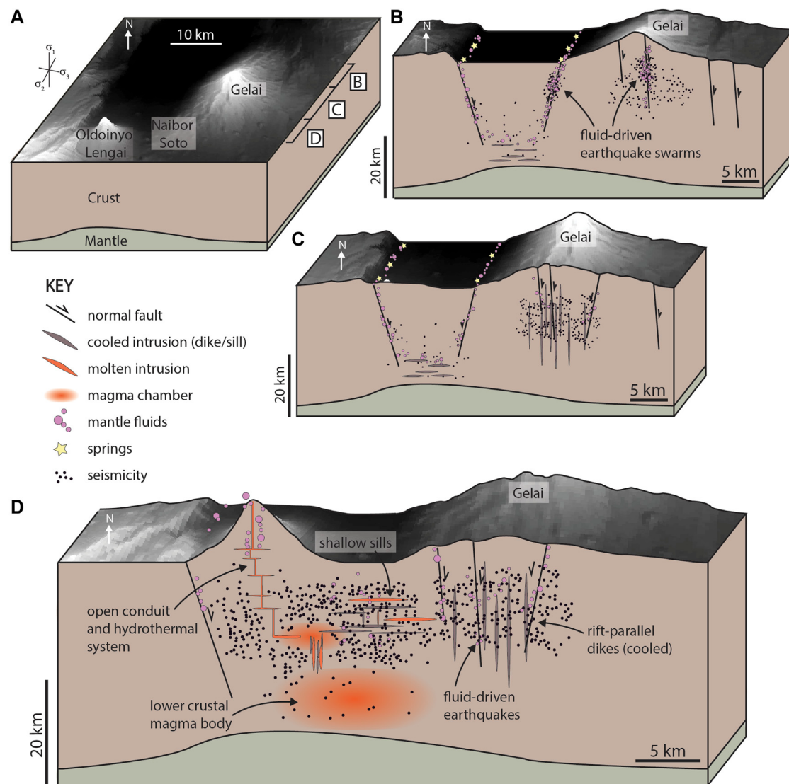
FIGURE 13 | Idealized conceptual illustration of magmatic-fluid-tectonic interactions associated with the volcanic plumbing system of the south Natron basin. The structure of the plumbing systems is based on data and interpretations presented in the current study, as well as previous seismicity and geophysical studies by Roecker et al. (2017) and Weinstein et al. (2017). Crustal thicknesses are broadly based on Plasman et al. (2017) and surface topography is from the 90 m SRTM DEM dataset. (A) Surface topography and general crustal structure of the south Natron basin, highlighting the position of the key volcanic features. Letters refer to the presented crustal sections in (B–D) . (B) General distribution of seismicity at the northern end of the seismic network. Deep seismicity occurs below Lake Natron, with seismic swarm behavior associated with fluid overpressures and fluid migration through the crust. Helium isotope data of dissolved spring volatiles and carbon isotopes of diffusely degassing \text{CO}_2 support mantle fluid flow through these fault systems (Lee et al., 2016; Lee et al., 2017; Muirhead et al., 2020). (C) General distribution of seismicity through central regions of the seismic network. Seismicity patterns generally follow those in B and support fluid-driven earthquakes, although no specific seismic swarms have been identified. Cooled dike intrusions represent regions of past magmatic rifting, although no significant melt or active diking is inferred below Gelai volcano currently. (D) General distribution of seismicity throughout the southern end of the seismic network, with deformation patterns strongly influenced by the presence of melt and fluids. The infrequent occurrence of seismicity in the lower crust below the Naibor Soto volcanic field support the presence of lower crustal magma bodies, consistent with the crustal velocity structure presented by Roecker et al. (2017). Distinct seismic gaps below these volcanic systems represent vertical zones of partial melt and/or thermally altered regions, and represent possible connections between partial melt bodies at different crustal depths (Weinstein et al., 2017). Melt bodies and topographic loads impose local stress perturbations (Oliva et al., 2019b) indicated by variations in fault plane solutions observed in this system. Persistent low magnitude seismicity throughout the region supports a model of earthquake activity driven by the percolation of melt and magmatic volatiles, consistent with full moment tensor analyses by Oliva et al. (2019a) who found various non-double couple earthquake source mechanisms.
