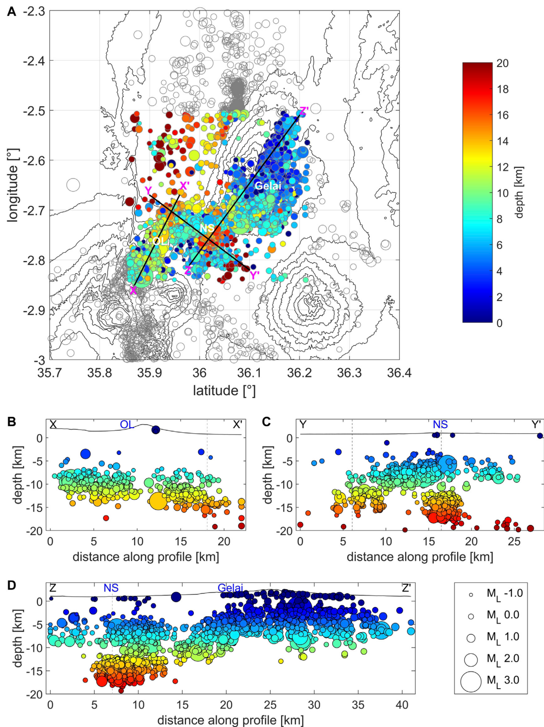
FIGURE 5 | (A) Map view of well-located earthquakes scaled by their magnitude and colored by their depth. (B) Enlarged vertical cross-section along the profile of X-X'. (C) Enlarged vertical cross-section along the profile of Y-Y'. (D) Enlarged vertical cross-section along the profile of Z-Z'. Intersections between profiles are marked with a gray dashed line. Color scale is saturated at 20 km for better visibility, as few events occur beneath 20 km depth.
