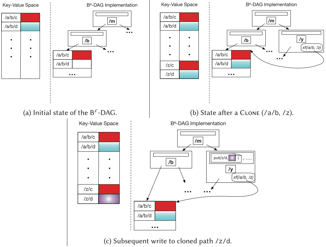
Fig. 3. The state of a B^E -DAG before and after a CLONE ( /a/b, /z ), which logically copies the keys and values with prefix /a/b , replacing the prefix with /z . This is implemented as a DAG, by adding a translation prefix (x) and filter (f), or xf function, to a child pointer in the DAG. The xf function ignores any key-value pairs in the node that do not match the source prefix (in this case, /a/b ).
