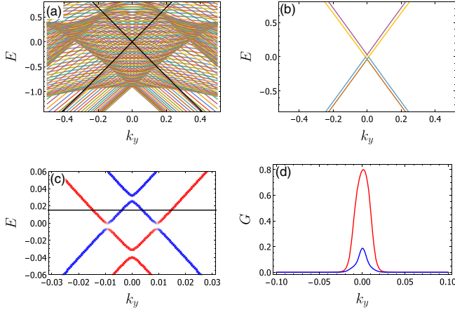
FIG. 4. Results of the tight-binding calculation. (a),(b) The graphene-WSM spectrum is shown near the \mathbf{K} and the \mathbf{K}' valleys, respectively. The Dirac cone in the \mathbf{K} valley (shown in black) is immersed in the bulk states of the WSM, while the Dirac cone near the \mathbf{K}' valley is slightly perturbed. (c) An expanded view of the \mathbf{K}' valley shows an inverted band structure where the colors code the average of S_z operator, with red being spin up and blue spin down. (d) The conductance of the graphene-WSM device based on a simplified model for the states near the \mathbf{K}' valley is shown in units of e^2/h . The conductance shows partial spin polarization as red denotes spin up states, where blue denotes spin down states.
