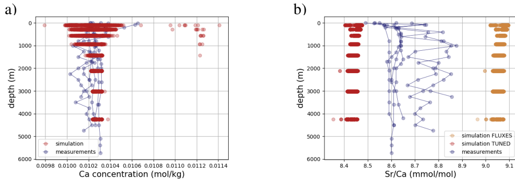
Figure B8. Comparison between measured and simulated Ca and Sr/Ca profiles in seawater. Shown are composites of all available measured concentration profiles and all profiles in the simulation. Data is taken from Fabricand et al. (1967), De Villiers (1999) and Fantle and Tipper (2014). Ca concentrations are normalized to a salinity of 34.90 PSU.
