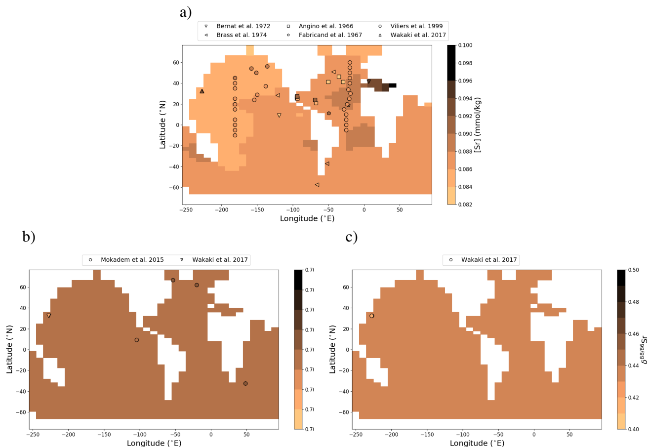
Figure C1. Comparison between measured and simulated Sr concentrations and isotopic composition in surface waters. Measurements are shown as symbols on the map, the colour indicating the respective value. Data is taken from Angino et al. (1966), Fabricand et al. (1967), Bernat et al. (1972), Brass and Turekian (1974), De Villiers (1999), Mokadem et al. (2015) and Wakaki et al. (2017).
