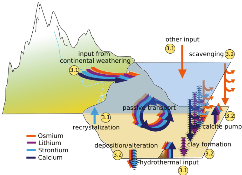
Figure 2. Processes included in the cGENIE trace metal implementation and the number of the subsection describing their implementation. Hashed arrows indicate processes during which isotopic fractionation occurs in the model.
