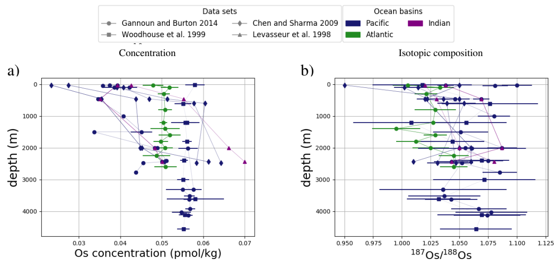
Figure B2. Measured Os ocean profiles. Shown are composites of all available profiles of measured concentrations and isotopic compositions. Data are taken from Levasseur et al. (1998), Woodhouse et al. (1999) and Gannoun and Burton (2014).
