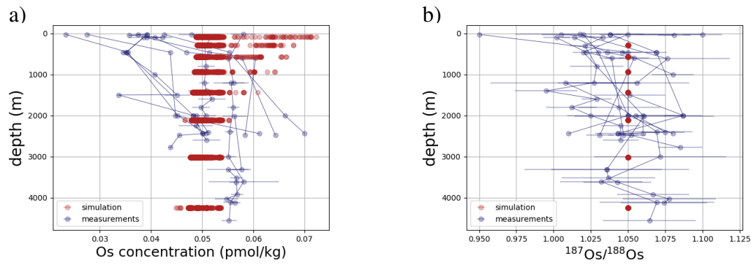
Figure B6. Comparison between measured and simulated Os vertical profiles in seawater. Shown are composites of all available measured Os concentration and isotope ratio profiles and all profiles in the simulation. Data is taken from Levasseur et al. (1998), Woodhouse et al. (1999) and Gannoun and Burton (2014).
