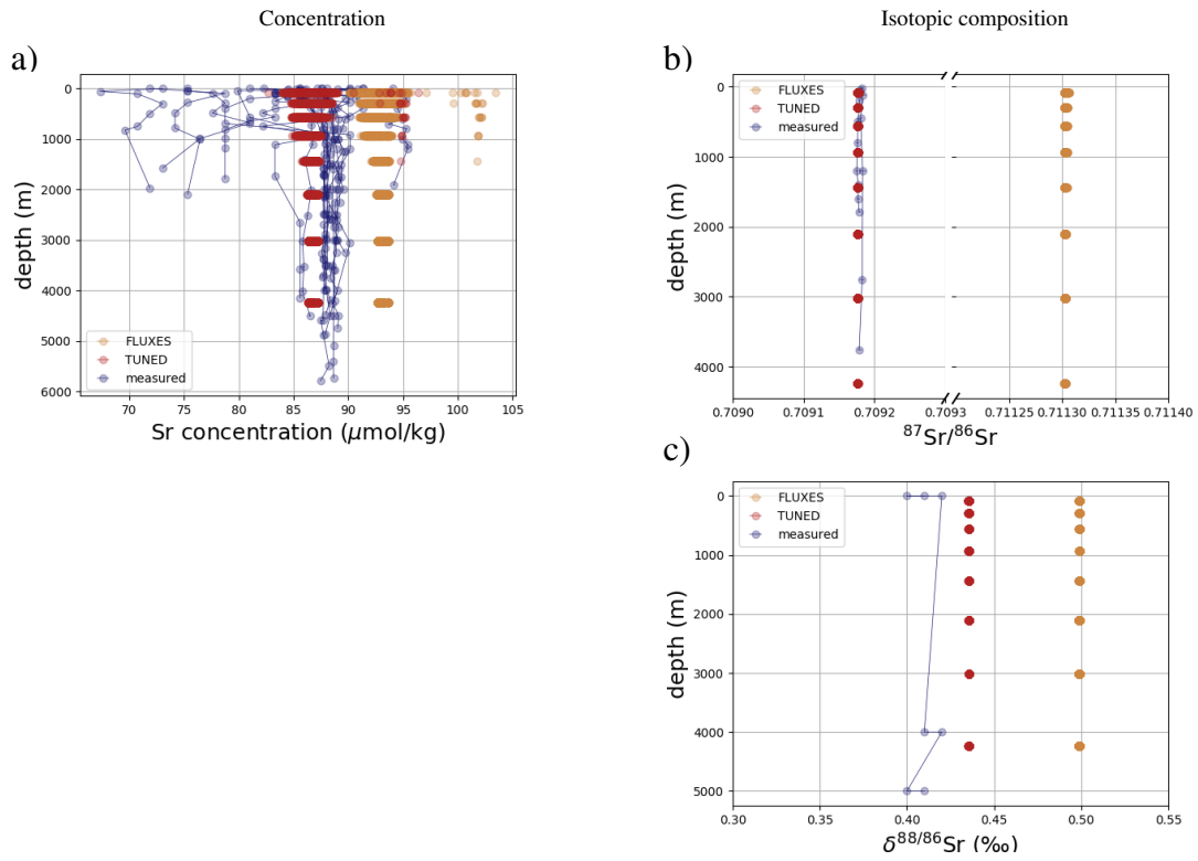
Figure B5. Comparison between measured and simulated Sr profiles in seawater. Shown are composites of all available measured Sr concentration and isotope ratio profiles and all profiles in the simulation. Data is taken from Angino et al. (1966), Fabricand et al. (1967), Bernat et al. (1972), Brass and Turekian (1974), De Villiers (1999) and Mokadem et al. (2015). Sr concentrations are normalized to a salinity of 34.90 PSU.
