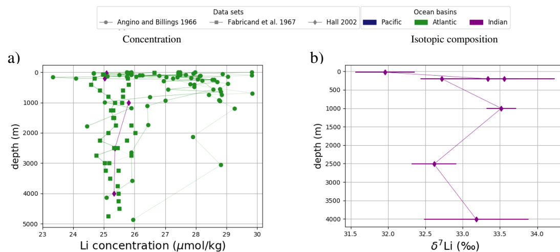
Figure B3. Measured Li ocean profiles. Shown are composites of all available profiles of measured concentrations and isotopic compositions. Data are taken from Angino and Billings (1966), Fabricand et al. (1967), Chan (1987) and Hall (2002). Li concentrations are normalized to a salinity of 34.903495.
