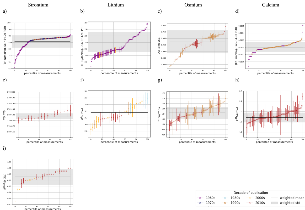
Figure 1. Sr, Li, Os and Ca composition of modern seawater. Shown are composites of all published measured concentrations and isotope ratios with reported errors. From these, we calculated mean concentrations and isotope ratios weighted by the reported error (the more uncertain a value, the less it contributes to the mean), which are indicated by horizontal lines. Shading indicates one weighted standard deviation around the means. Data are taken from Angino et al. (1966), Fabricand et al. (1967), Bernat et al. (1972), Brass and Turekian (1974), De Villiers (1999), Pearce et al. (2015), Mokadem et al. (2015) and the compilation of Wakaki et al. (2017) for Sr, Angino and Billings (1966), Fabricand et al. (1967), Chan (1987), Chan and Edmond (1988), You and Chan (1996), Moriguti and Nakamura (1998), Tomascak et al. (1999), James and Palmer (2000), Košler et al. (2001), Nishio and Nakai (2002), Hall (2002), Bryant et al. (2003), Pistiner and Henderson (2003), Millot et al. (2004), Choi et al. (2010), Pogge von Strandmann et al. (2010), Phan et al. (2016), Lin et al. (2016), Henchiri et al. (2016), Weynell et al. (2017), Fries et al. (2019), Gou et al. (2019), Hindshaw et al. (2019), Murphy et al. (2019) and Pogge von Strandmann et al. (2019b) for Li, Levasseur et al. (1998), Woodhouse et al. (1999) and Gannoun and Burton (2014) for Os and Fabricand et al. (1967), De Villiers (1999) and Fantle and Tipper (2014) for Ca. The decade of publication is indicated by colour as measurement techniques for some metals/isotopes have improved over time. Concentrations of Sr, Li and Ca are normalized to a salinity of 34.90 PSU. Os concentrations could not be salinity-normalized because of missing salinity measurements at one out of three measurement sites (Woodhouse et al., 1999).
