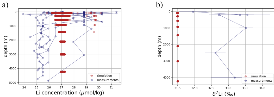
Figure B7. Comparison between measured and simulated Li profiles in seawater. Shown are composites of all available measured Li concentration and isotope ratio profiles and all profiles in the simulation. Data is taken from Angino and Billings (1966), Fabricand et al. (1967), Chan (1987), Chan and Edmond (1988), You and Chan (1996), Moriguti and Nakamura (1998), Tomascak et al. (1999), James and Palmer (2000), Košler et al. (2001), Nishio and Nakai (2002), Hall (2002), Bryant et al. (2003), Pistiner and Henderson (2003), Millot et al. (2004), Choi et al. (2010) and Lin et al. (2016). Li concentrations are normalized to a salinity of 34.90 PSU.
