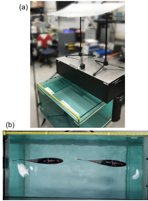
Figure 5: (a) Experimental setup showing the water tank and an overhead camera setup (with a light diffuser) to estimate the swimming speed. (b) Two time instances of the swimming robotic fish.
