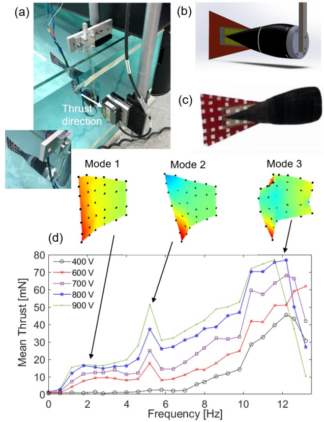
Figure 9: (a) Experimental setup for hydrodynamic thrust measurement in quiescent water. (b) CAD model and (c) a photo of the part of the second generation robotic fish body used in the thrust measurement tests with (reflector tapes are for LDV measurements). (d) Mean thrust frequency response for different actuation voltage amplitude levels over a frequency range covering the first three vibration modes.
