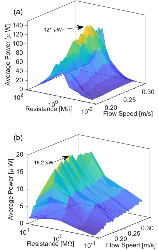
Figure 12: Average electrical power versus load resistance and flow speed for a bluff body diameter of (a) d_0=25.4 mm and (b) d_0=15.9 mm ( d = 2.5d_0 was used in each case for the distance between the center of the bluff body and the tail tip).
