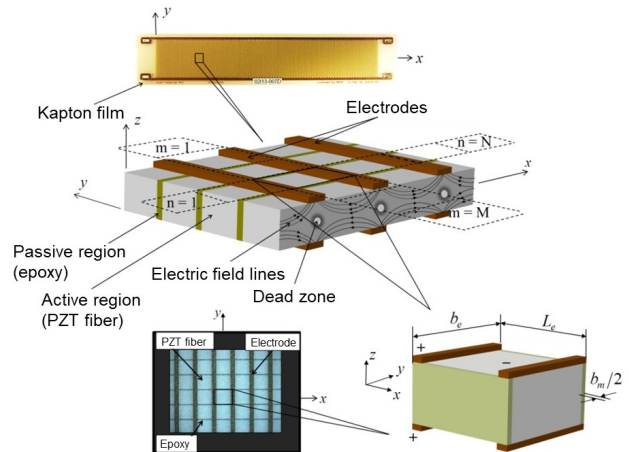
Figure 1: Detailed view of a single MFC laminate (M8514-P1 model is shown as an example) displaying piezoelectric fibers and interdigitated electrodes embedded in a Kapton film. Polyester electrode sheets (custom made by the manufacturer - Smart Material Corp.) enable waterproofing.
