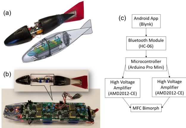
Figure 4: (a) Fully constructed robotic fish along with (b) a close-up view of its electronics and (c) a summary of the components involved in dynamic actuation of the piezoelectric tail.
