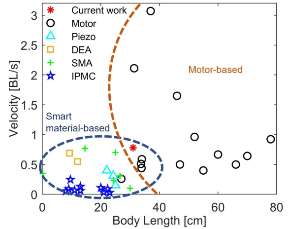
Figure 14: Performance comparison of smart material-based and motor-based untethered robotic fish. Current generation swimmer is at the intersection of these actuators, offering both geometric scalability and high performance.
