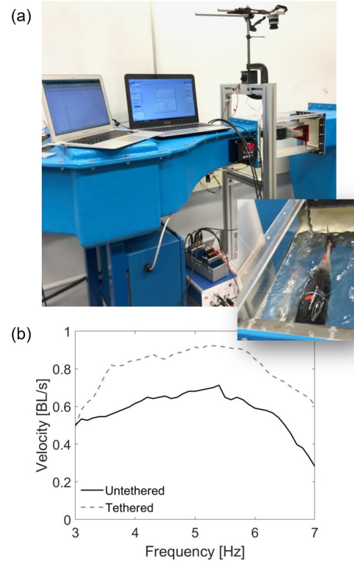
Figure 8: (a) Water tunnel used for the experiments with imposed flow with a close-up view of the test section. (b) Steady-state velocity of the robotic fish versus tail actuation frequency as measured in the water tunnel for untethered (battery powered) and tethered configurations.
