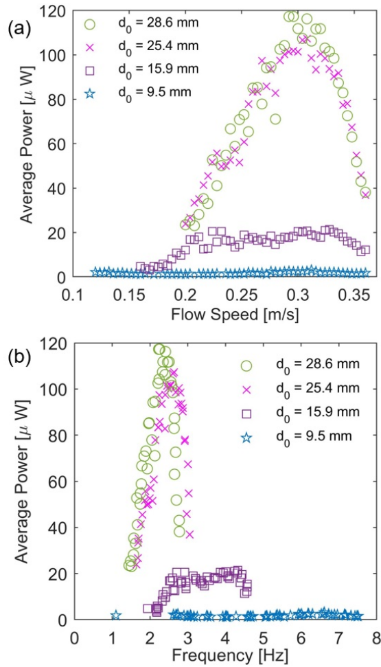
Figure 13: Average electrical power (a) versus flow speed and (b) versus shed vortex frequency for different bluff body diameters.
