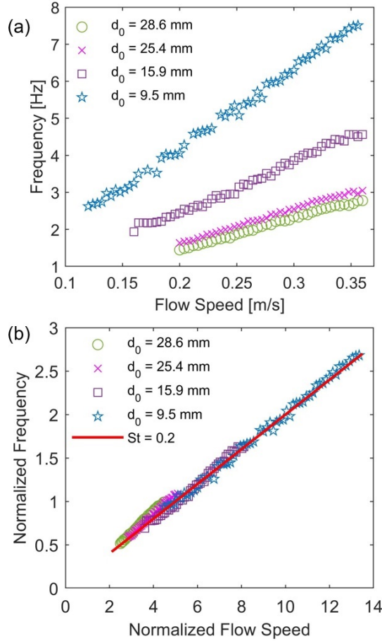
Figure 11: (a) Shed vortex frequency versus flow speed obtained for a number of bluff body diameters and (b) its dimensionless version with vortex frequency normalized by the first resonance frequency and flow speed normalized by the bluff body diameter and first resonance frequency (which is accurately represented by the solid line with a slope of St = 0.2 due to the relationship f = St \frac{U}{d_0} ).
