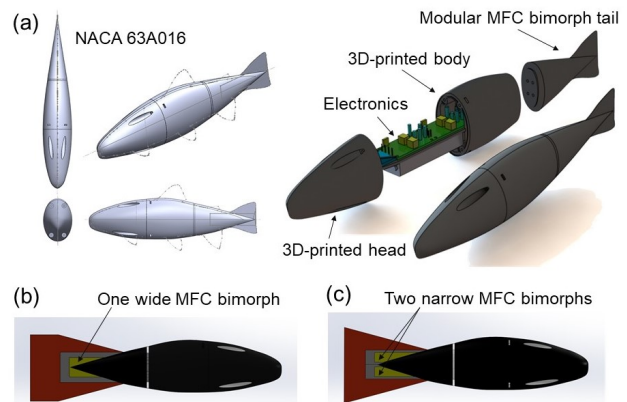
Figure 2: (a) CAD model and 3D views of the trout-like robotic fish (based on NACA 63A016 airfoil) and its basic components. Two generations of the modular tail using (b) one pair of wide MFCs (first generation) and (c) two pairs of narrow MFCs (second generation) sandwiching the passive fin.
