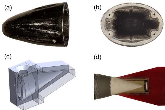
Figure 3: Various components of the fish body and details of the manufacturing process: (a) 3D-printed nose with a thin coat for waterproofing. (b) Gasket at the 3D-printed main body and nose intersection. (c) CAD model of the 3D-printed mold to fabricate the silicone portion of the tail. (d) Tail assembly (first generation) after vacuum bonding a pair of wide MFCs to PVC fin and combining with silicone in the mold.
