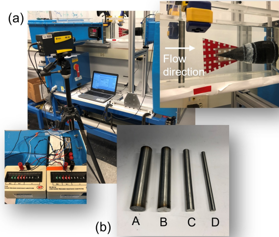
Figure 10: (a) Experimental setup for energy harvesting from the wake of a cylindrical bluff body with a close-up view of the test section and electrical load boxes. (b) Bluff body samples (cylinders) with different diameters, A: 28.6 mm, B: 25.4 mm C: 15.9 mm D: 9.5 mm.
