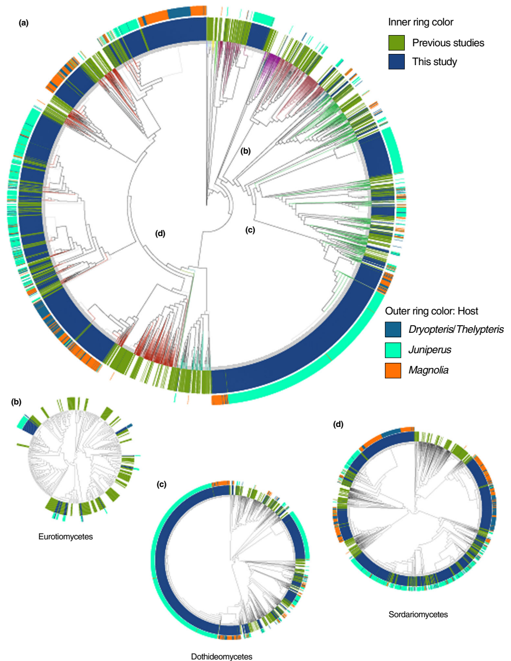
Fig. 5 Phylogenetic placement of cultured endophytes in this study with representative sequences from each OTU from 45 previous studies (Supplementary Table 1) and 1625 reference taxa in the Pezizomycotina, as determined using T-BAS [67]. All isolates of a given OTU obtained in this study and one representative per OTU from the previously published data are shown in tips of branches. OTUs are based on 95% sequence similarity. (a) Pezizomycotina tree, and (b–d) represent three major classes of Pezizomycotina that contained the majority of endophyte isolates from this study (See Fig. 4). The settings to place the sequences from this study and previous studies were UNITE filter engaged, no clustering for visualizing purpose, 10 standard deviation as genetic distance cutoff, and likelihood weights with the outgroup selected in RAxML options. Reference taxa are shown with colored branches (colored by class), with no color in the inner and outer ring in (a)
