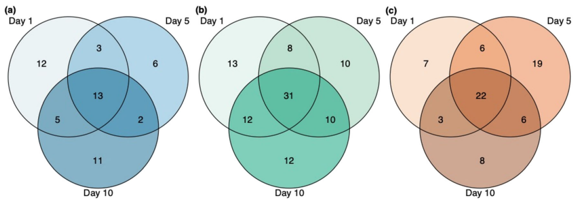
Fig. 3 The number of unique species at each storage periods and of shared species among storage periods in (a) Dryopteris/Thelypteris , (b) Juniperus , and (c) Magnolia in culture-based data set. Cultures from five media were pooled. Endophyte community structure based on presence/
