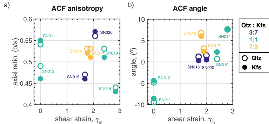
Figure 13. SPO data on the shear zone scale. (a) Shear strain versus ACF anisotropy. (b) Shear strain versus orientation of ACF ellipses. SPO, shape preferred orientation; ACF, autocorrelation function.
