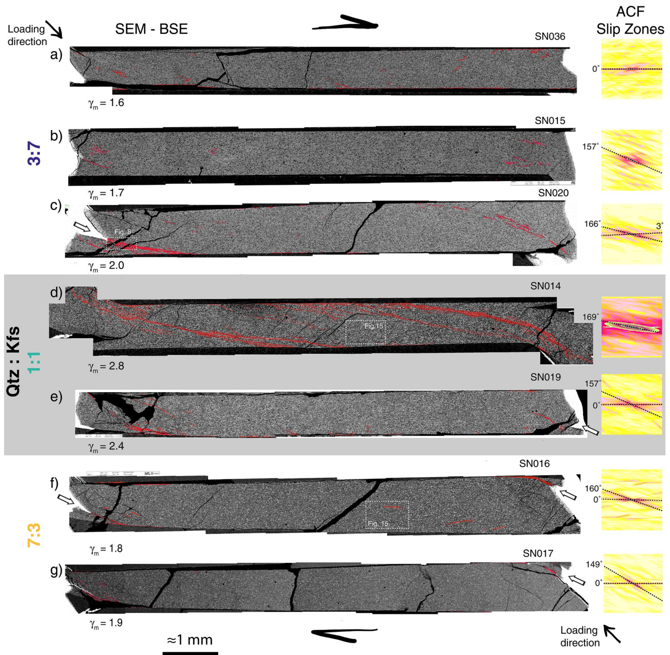
Figure 7. SEM-BSE images of deformed samples showing the slip zone geometry (red tracings) on the sample scale. (a–c) 3:7, (d and e) 1:1, and (f and g) 7:3 Qtz:Kfs ratio samples. Most of the slip zones originate at the boundaries of the shear zone and propagate inward with increasing strain. Experiments sheared to \gamma > 2 have developed the most connected slip zones (high fractal dimension D ). White arrows highlight the protrusion of the gold jacket (white) into the fault rock marking the presence of a slip zone. The average angle of propagation of the slip zones is estimated by measuring the dominant orientations of the ACF on the right. White dashed rectangles show location of high-magnification SEM images and EBSD maps shown in subsequent figures. SEM-BSE, scanning electron microscope-backscatter electron; ACF, autocorrelation function; EBSD, electron backscattered diffraction.
