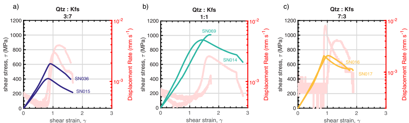
Figure 3. Mechanical data for constant displacement rate experiments: stress-strain curves. Shear stress versus strain and \sigma_1 piston displacement rate (red curves) for (a) 3:7, (b) 1:1, and (c) 7:3 Qtz:Kfs ratio samples.
