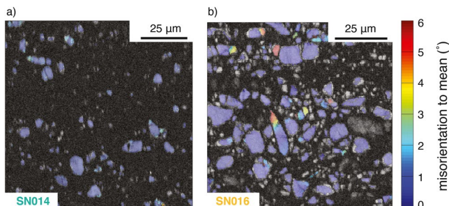
Figure 16. Misorientation with respect to mean orientation (mis2mean) within grains. Band contrast image as background.
