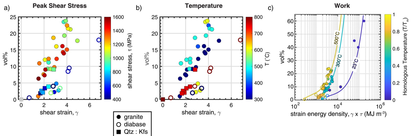
Figure 17. The volume of the slip zones from our experiments with the data from Pec, Stünitz, and Heilbronner (2012), Pec, Stünitz, Heilbronner, Drury, et al. (2012), Pec et al. (2016), Marti et al. (2017, 2020), and Yund et al. (1990) color coded for different conditions. Solid circles are for granitic rocks, empty circles are for diabase and squares for Qtz:Kfs aggregates. (a) The effect of peak shear stress on the vol% of the slip zones. (b) The effect of temperature on the vol%. (c) Illustrates the effect the strain energy density on the vol% of slip zones normalized to homologous temperature. Curves show the least squares fits to the granite data.
