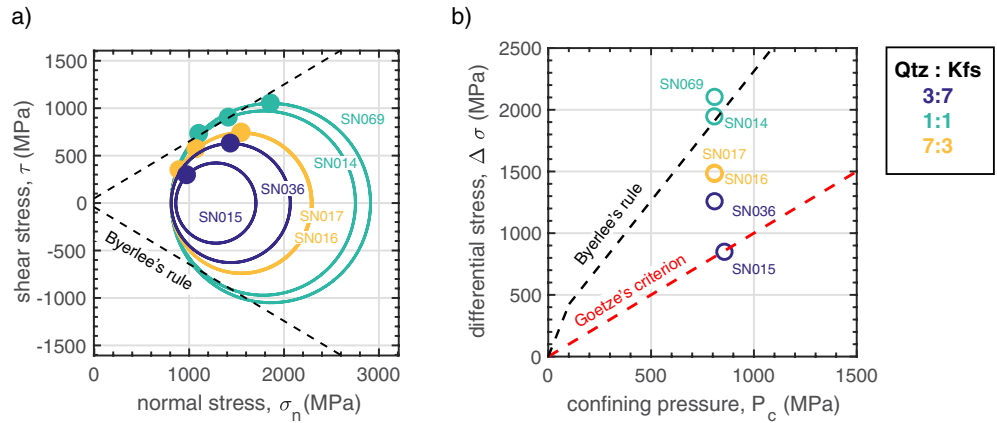
Figure 4. Mechanical data from constant displacement rate experiments: Mohr space. (a) Mohr circles at peak strength, dashed line represents Byerlee's rule. Full circles show measured orientations of slip zones (see text for details). (b) Data from all experiments plotted in a differential stress versus confining pressure space.
