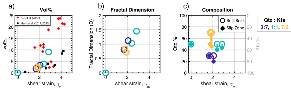
Figure 11. Summary of microstructural data from the slip zones. (a) Volume of slip zones versus shear strain shows a strong positive correlation. Red and black symbols show measurements from different studies performed at similar conditions, see text for details. (b) Fractal dimension of slip zones: fractal dimension (i.e., complexity of the pattern) increases with increasing strain. (c) Change in mineralogy within slip zones. In all samples, the slip zones are depleted in Qtz with respect to the bulk rock. Samples with an initial Qtz:Kfs ratio of 7:3 show the most significant change.
