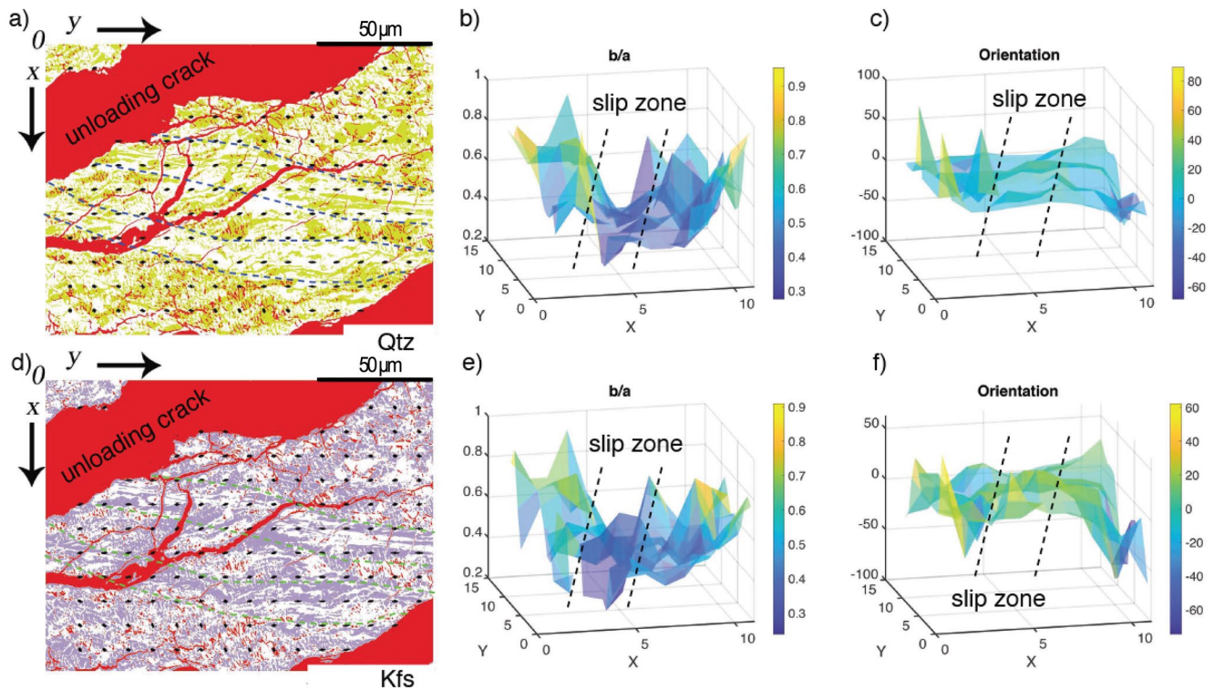
Figure 10. Tessellation of ACF squares surrounding a slip zone. (a and d) ACF ellipses are plotted on the top of binary Qtz and Kfs images, respectively. Dashed lines highlight slip zones. Red background color represents unloading cracks. (b and e) SPO anisotropy: axial ratio ( b/a ) of each phase plotted in a 3D plot. The slip zone has a higher anisotropy (lower b/a ratio) than the rest of the sample. (c and f) ACF orientation. Inside the slip zones, the orientation is approximately zero (parallel to the shear zone boundary). ACF, autocorrelation function; SPO, shape preferred orientation.
