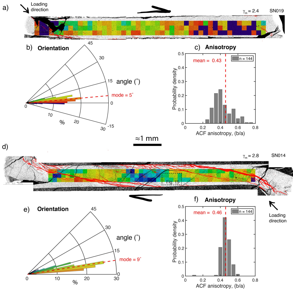
Figure 14. ACF tessellation analysis of 144 squares covering large portions of the shear zone from unsegmented SEM-BSE images in 1:1 Qtz:Kfs ratio samples. (a) Constant load sample. (b) ACF orientation rose diagram (colors in histogram correspond to colors of squares in (a)). (c) ACF anisotropy histogram. (d) Constant displacement rate sample. (e) ACF orientation rose diagram (colors in histogram correspond to colors of squares in (a)). (f) ACF anisotropy histogram. ACF, autocorrelation function; SEM-BSE, scanning electron microscope-backscatter electron.
