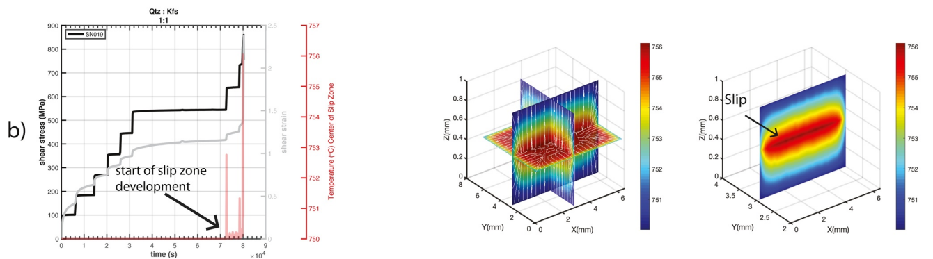
Figure 18. Heat flow simulation of experiment SN019. (a) A plot of stress, strain rate, and temperature versus time. Temperature is plotted for the center of the sample. Right figures display the end-time temperature distribution on cross sections of the cube. (b) Temperature versus time with a slip zone introduced at the end of the experiment. The slip zone is introduced as a horizontal layer. The cross sections show the relative increase of temperature at the slip zone.
