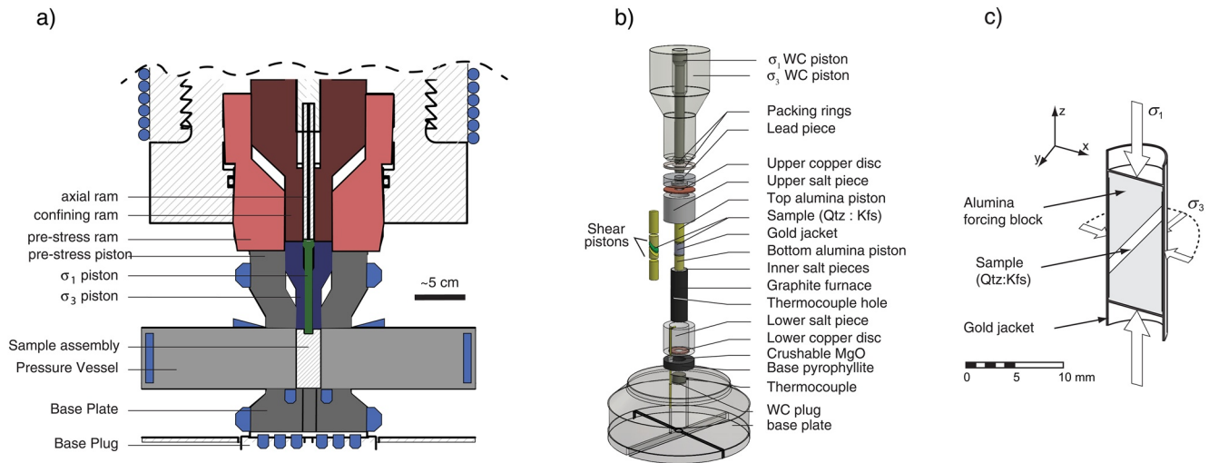
Figure 1. Schematic of experimental apparatus and the sample assembly. (a) Cross section of the Griggs-type apparatus. (b) Detailed schematic of the assembly components (modified after Précigout et al., 2018). (c) Geometry of the sample.
