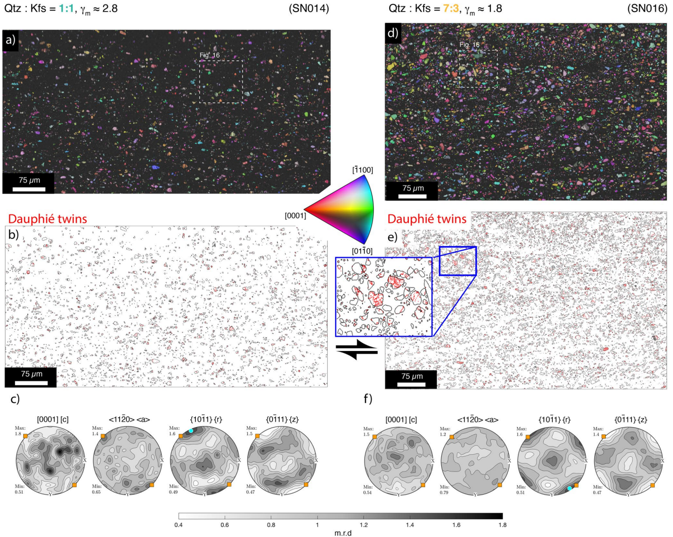
Figure 15. Summary of the EBSD analysis. (a and d) Orientation map of the Qtz grains color coded by the inverse pole figure (inset). Band contrast image shown in the background. White dashed rectangles show position of high-magnification data shown in Figures 16b and 16e. Dauphiné twin boundaries are shown in red. (c and f) Pole figures. Orange squares represent the loading direction and the cyan circle highlights the {r} axis maxima. Grain boundaries are in black. EBSD, electron backscattered diffraction.
