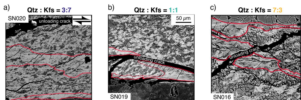
Figure 9. Representative slip zone microstructures from samples with different Qtz:Kfs ratios. Slip zones highlighted by red lines.
