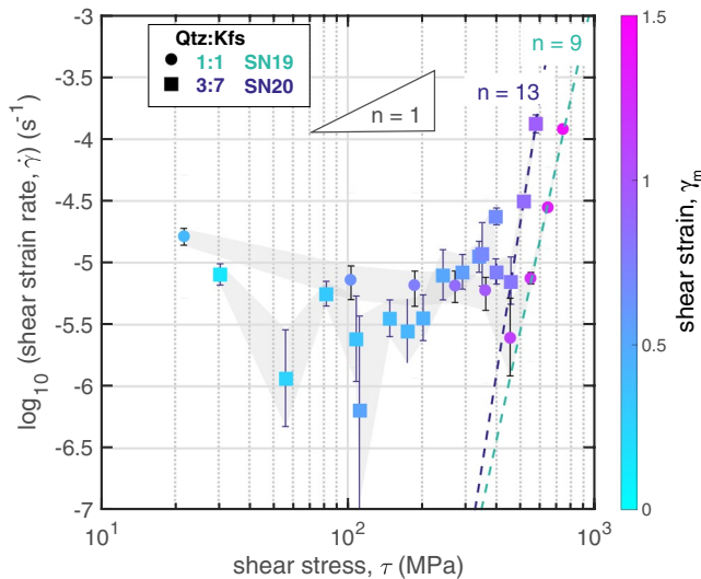
Figure 5. Mechanical data from constant load experiments: \log(\tau) versus \log(\dot{\gamma}) data color coded by mean strain at stress step. Error bars and shaded regions show 1 standard deviation (s.d.). The high strain rate at low stress ( <100 MPa) can be attributed to the early compaction of the samples. Notice that 1:1 Qtz:Kfs ratio samples are stronger than 3:7 Qtz:Kfs ratio samples and reach high stresses at higher strains (compare to Figure 3). Last three stress steps are fitted with a least squares linear fit and yield high-stress exponents ( n = 9 –13). See text for details.
