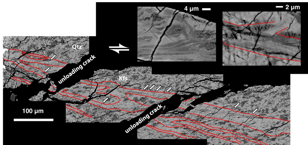
Figure 8. High-magnification image of a slip zone in a 3:7 Qtz:Kfs ratio sample (SN020). Image location within the sample shown in Figure 7. The slip zone is highlighted by red lines. White arrows highlight unloading cracks that concentrate in the slip zone material. Within the slip zone, notice the flow-like patterns and no resolvable grains or porosity on the field emission SEM scale. Insets show high-magnification images of slip zones illustrating the resolution of FE-SEM observations. Pores as small as \approx 20 nm can be reliably identified. SEM, scanning electron microscope.
