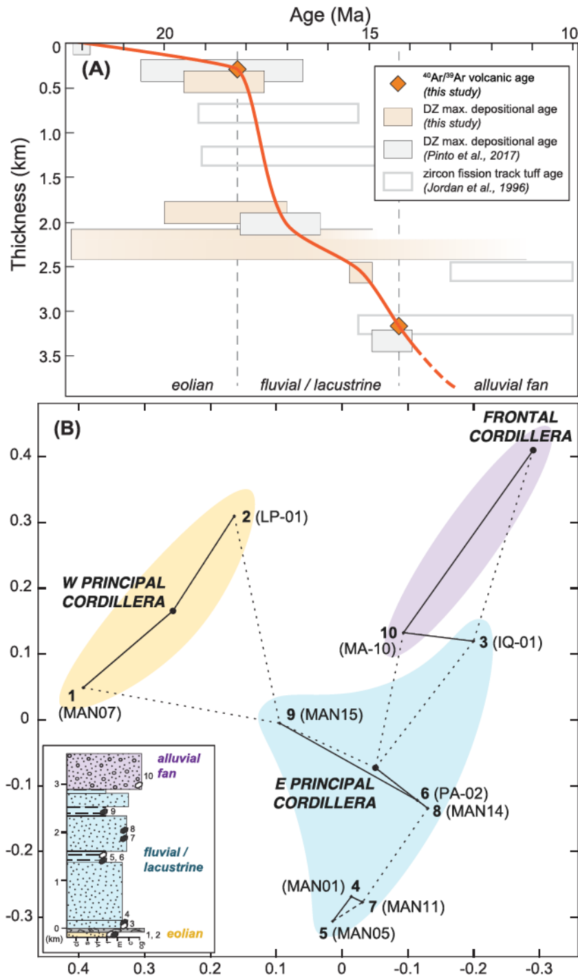
Fig 8. (a) Stratigraphic age versus thickness diagram for the Manantiales Basin. (b) Multidimensional scaling (MDS) plot showing relative statistical similarity (Komolgorov-Smirnov test D value; Vermeesch, 2013) between Manantiales Basin detrital zircon samples and composite zircon age distributions representative of potential sediment sources (Western Principal Cordillera, Eastern Principal Cordillera, and Frontal Cordillera; Mackaman-Lofland et al., 2019; Pinto et al., 2018). Inset shows sample locations within the Manantiales section. Symbols are explained in Figure 3.
