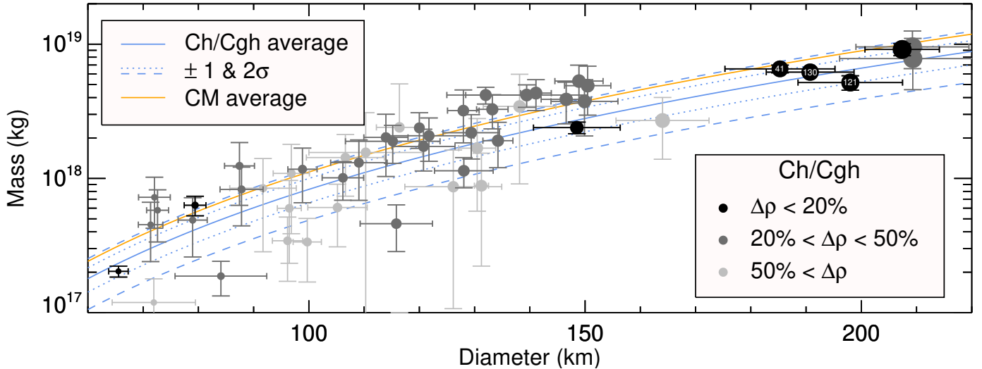
Fig. 4. Mass vs. diameter distribution for 76 Ch/Cgh asteroids (grey circles). Those more precise than 50 and 20% are plotted as dark grey and black circles, respectively. Unreliable density estimates (below 0.5 \text{ g cm}^{-3} ) are not displayed. The three binary asteroids, (41) Daphne, (121) Hermione, (130) Elektra, are labeled. The solid and dashed blue curves represent the average density ( 1.58 \text{ g cm}^{-3} ) and 1\sigma – 2\sigma ( \pm 0.33 \text{ g cm}^{-3} ) dispersion of the sample. The solid orange curve stands for the average density of CM chondrites at 2.13 \pm 0.57 \text{ g cm}^{-3} ( 3\sigma ).
