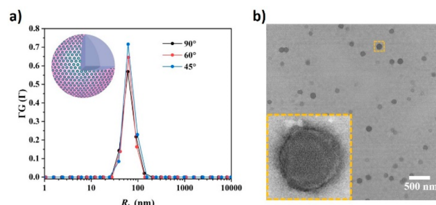
Figure 6. (a) DLS results of a solution of 1 , \{\text{Mo}_{90}\text{Ce}_{10}\} (40 equiv of BaCl 2 ) at different scattering angles. The R_h value is 62(\pm 5) nm. (b) TEM images obtained from \{\text{Mo}_{90}\text{Ce}_{10}\} solution with 40 equiv of BaCl 2 .
