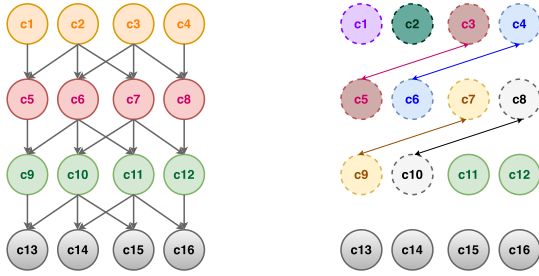
(a) A DAG job with 16 coflows. (b) Scheduling of coflows.
