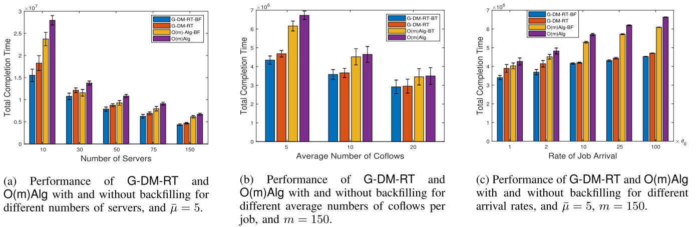
Fig. 6. Performance of G-DM-RT and O(m)Alg for scheduling rooted tree jobs with and without backfilling.
