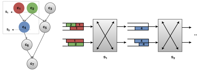
(a) A multi-stage job with 7 coflows. (b) Flows of coflows 1, 2, and 4 and their dependencies in a 2 \times 2 switch.
