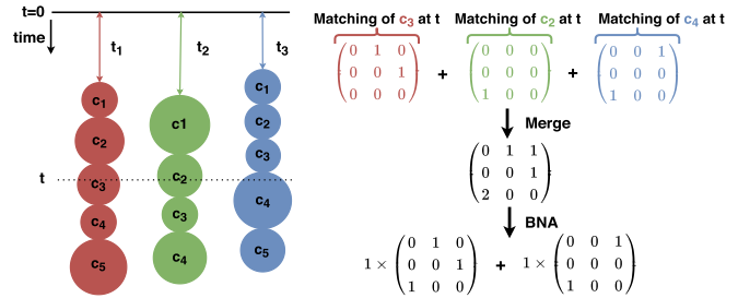
Fig. 2. Applying DMA on 3 multi-stage jobs. On the left side, a topological ordering and a random delay for each job are computed. On the right side, the merging procedure and BNA output is shown for some time t .
