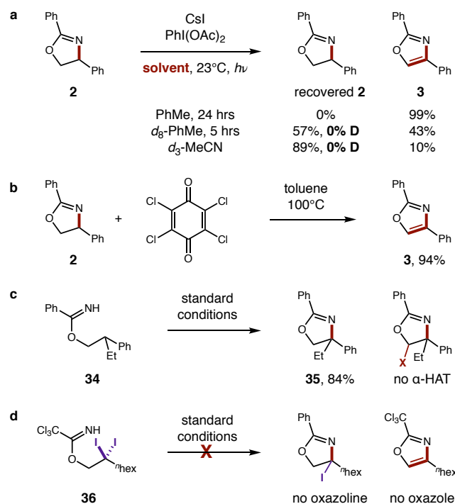
Fig. 9. Mechanistic evaluation of second HAT.
