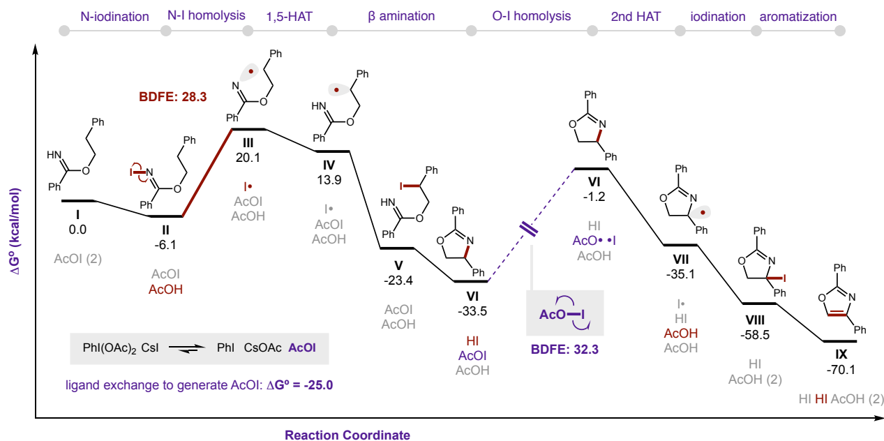
Fig. 11. Gibbs free energies of reaction intermediates. \omega B97X-D/6-311++G(d,p)/Def2-TZVPP(I and Cs)/PCM(PhMe).
