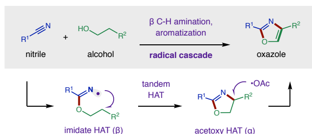
Fig. 1 Azole synthesis via tandem hydrogen atom transfer.
