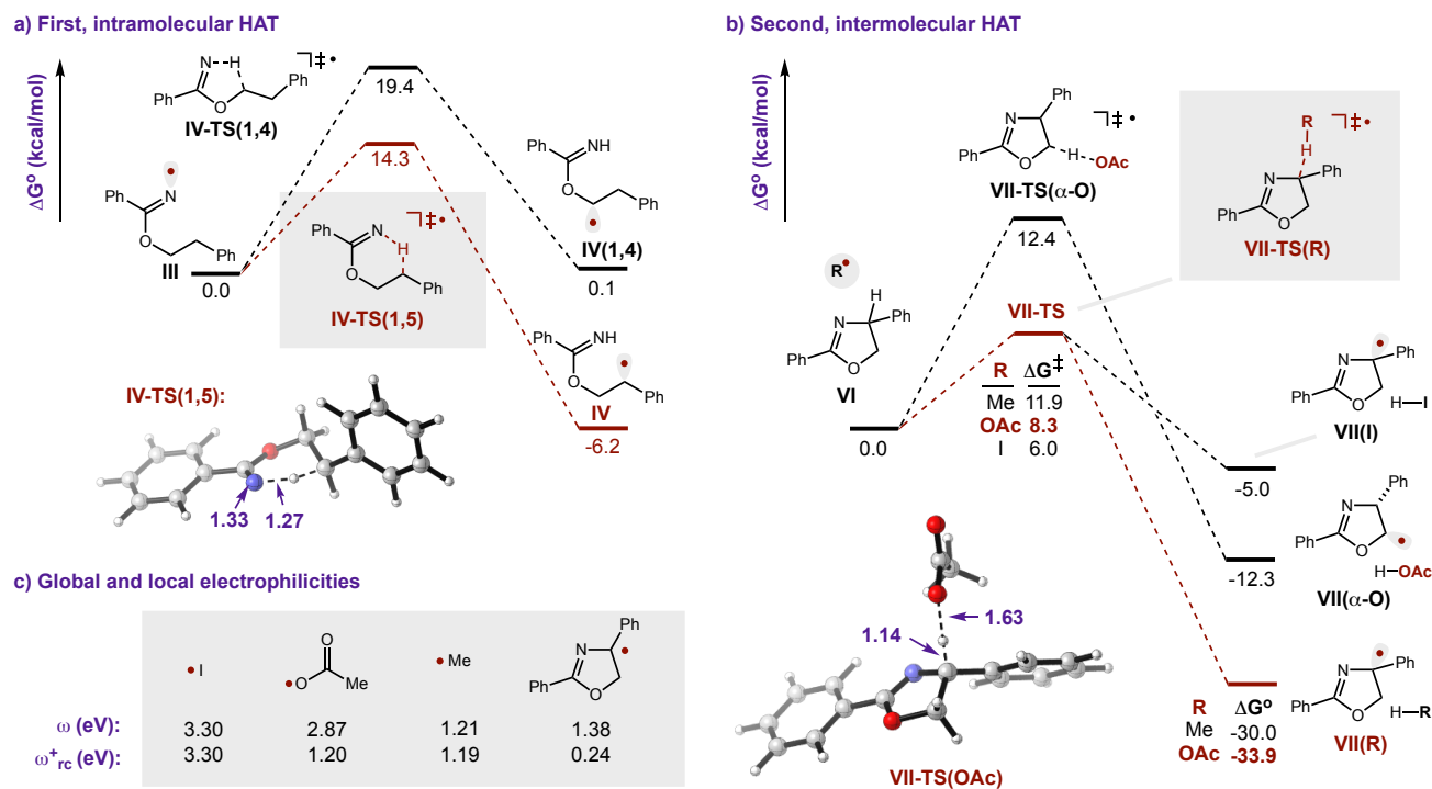
Fig. 12. Energetics of HAT steps. a) 1,5 vs 1,4 HAT. b) Intermolecular HAT pathways. Selected TS bond lengths in angstroms, Å. c) Global and local electrophilicities of key radicals. \omega B97X-D/6-311++G(d,p)/Def2-TZVPP(I)/PCM(PhMe).
