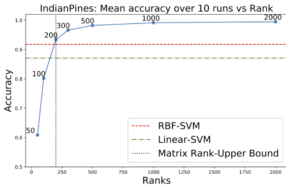
Fig. 2. Mean accuracy vs. Rank of the tensor observed over 10 runs. As rank increases, the classification accuracy increases and stabilizes after a certain point.
