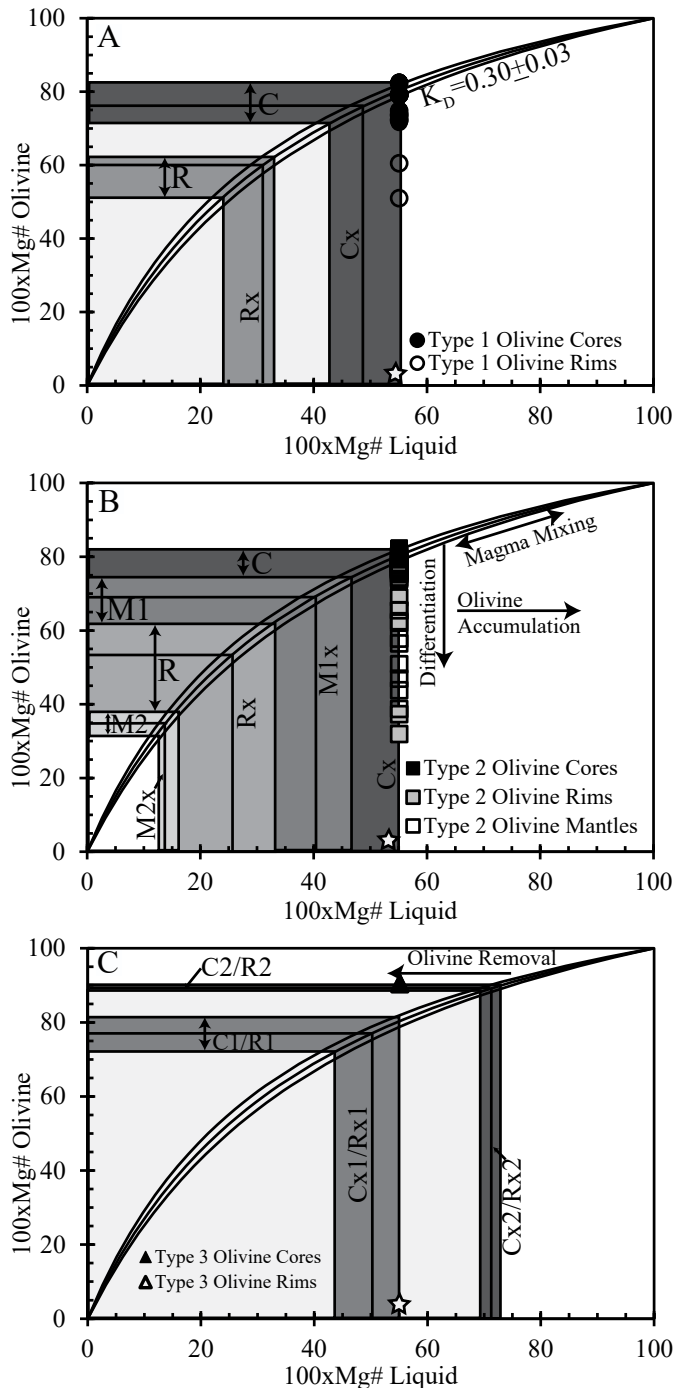
FIGURE 5. Mg#-olivine versus Mg#-liquid for olivine from the McCartys Flow. A-C) Inferred equilibrium-melt composition (Mg#) from measured olivine composition (Fo#), using Fe-Mg partition coefficients divided by olivine phenocryst type. Labeled arrows show schematically the effects of olivine accumulation and crystallization. Olivine cores from phenocryst types 1 and 2 are considered in equilibrium with the melt as represented by the whole-rock composition. Type 3 olivine phenocrysts are the result of olivine removal from a more primitive composition melt. Type 2 mantles and rims from olivine types 1, 2, and 3 are the result of olivine crystallization during melt differentiation. Rims, cores, and mantle data are separated and shown as the range in compositions found (arrows and grey shading). Means are marked by thick black lines inside the shaded area: Cx=mean core zone composition; Mx=mean mantle zone composition; and Rx= mean rim zone composition. Stars represent the whole rock composition.
