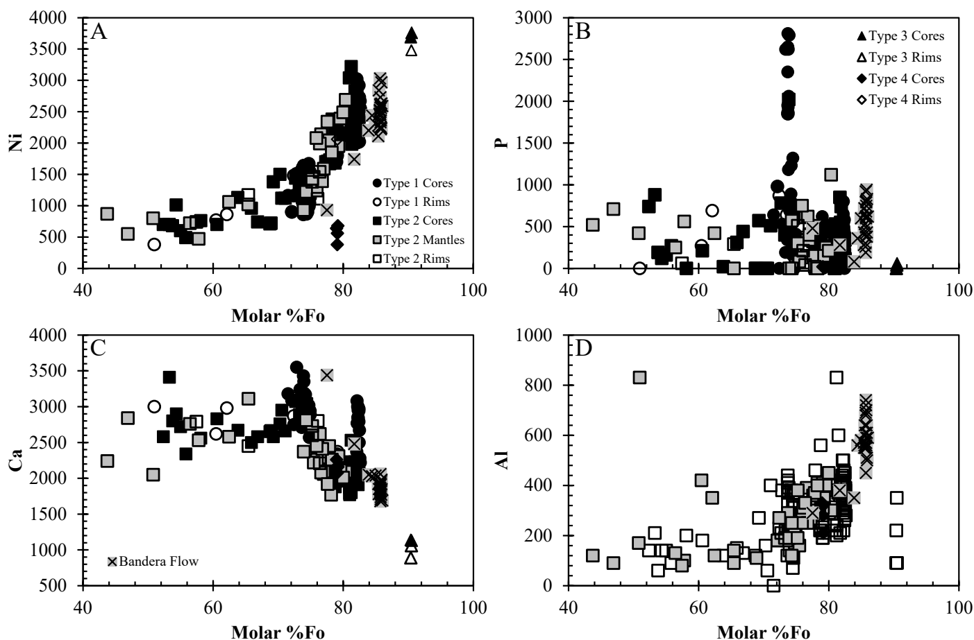
FIGURE 2. Variation diagrams for olivine phenocryst mineral chemistry from the McCartys and Bandera basalt flows. Trace elements are plotted against molar percent forsterite. McCartys Flow olivine are broken into crystal types described in text. Bandera Flow olivine phenocrysts are shown for reference and are homogeneous within a single crystal. Analytical uncertainties are equal to symbol size.
