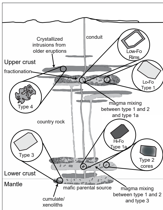
FIGURE 6. An integrated conceptual model of the basaltic magmatic conduit beneath the McCartys cinder cone explaining the textural and compositional characters of the olivine phenocrysts. The conceptual model is envisaged as a series of ephemeral conduits and chambers in space and time. Erupted basalts fractionate through a mafic parent in the lower crust or at the mantle-crust boundary accumulating or producing the \text{Fo}_{90} type 3 olivine. Type 1 (high-Fo#) and type 2 olivine cores ( \text{Fo}_{78-83} ) crystallize from the resulting basaltic melt in the lower crust. Type 2 olivine mantles are the result of further fractionation during magma ascent. During ascent, the basaltic magma encounters the crystallized remnants of previous plumbing systems which fed the older magmatic stages of the ZBVF and stalled crystal mush bodies in the mid to upper crust, entraining xenocryst type 4 olivine. Magma mixing between ascending magma with stalled magma mushes produce the \text{Fo}_{65} rims observed in type 1 and 2 olivine and new crystallization of euhedral \text{Fo}_{75} type 1 olivine phenocrysts. No lateral or vertical scale implied. Figure modified from Coote et al. (2019).
