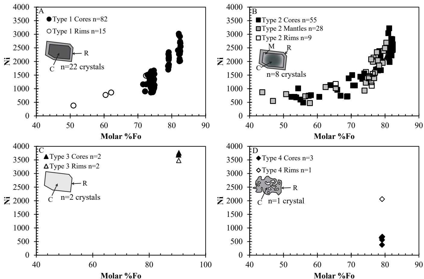
FIGURE 3. Nickel versus molar percent forsterite (Fo#) of McCartys Flow olivine phenocrysts. Analyses are divided by texture and by core, mantle, and rim analyses. A) Type 1 olivine are euhedral to subhedral crystals with homogeneous cores and lower Fo# and Ni-content rims. Core compositions fall into three general subgroups, \text{Fo}_{70-75} , \text{Fo}_{78-79} , and \text{Fo}_{81-82} . B) Type 2 olivine phenocrysts are euhedral to subhedral and contains core, mantle, and rims. Fo# and Ni contents decrease from core to rim for a single olivine phenocryst. Olivine phenocrysts from this group are found as individual crystals and in glomerocrysts with augite. C) Type 3 crystals are euhedral to subhedral crystals with homogeneous compositions. D) Type 4 olivine is anhedral with abundant olivine-hosted melt inclusions and melt embayments. Compositions are homogeneous for Fo# with rims containing higher Ni contents than the cores. Analytical uncertainties are equal to symbol size. C=core; M=mantle; R=rims.
