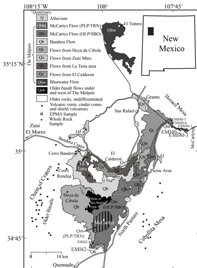
FIGURE 1. Location map of the Zuni-Bandera volcanic field showing the Bandera (Qb) and McCartys (Qm) flows and sample locations. Samples selected for olivine mineral chemistry are from the olivine-phyric basalt group and locations are shown by stars. Modified from Sims et al. (2007).
