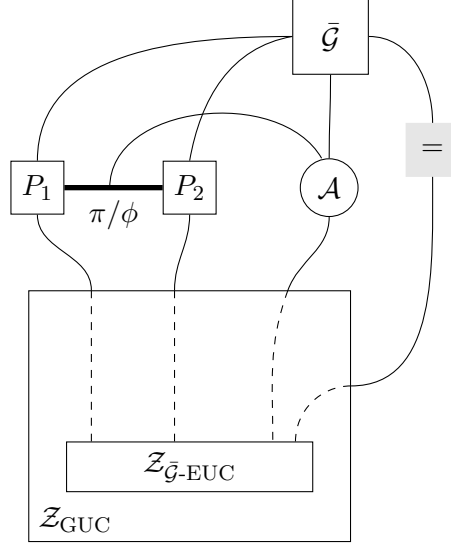
Figure 8: Constructing \mathcal{Z}_{\text{GUC}} out of \mathcal{Z}_{\bar{\mathcal{G}}\text{-EUC}} , where \text{=} denotes a dummy party.
