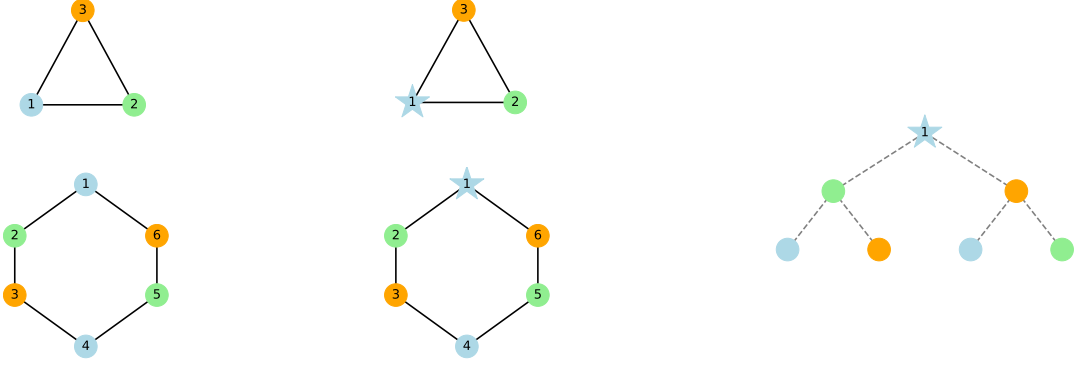
Figure 4: An illustration of rooted graphs and rooted aggregation trees. Left : a pair of graphs, G and G' . Center : the rooted graphs of 1 in G and G' , G^{[1]} and G'^{[1]} . Right : the rooted aggregation tree that both G^{[1]} and G'^{[1]} correspond to.
