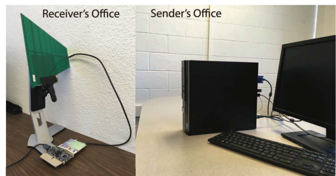
Fig. 5: Experimental setup for wall-penetrating performance evaluation
