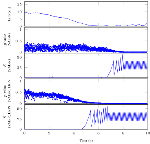
Fig. 7. Episode with dataset shift (label concept shift).
