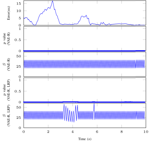
Fig. 5. Episode with dataset shift (covariate shift).
