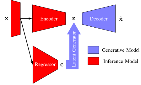
Fig. 2. VAE for regression model [14].
