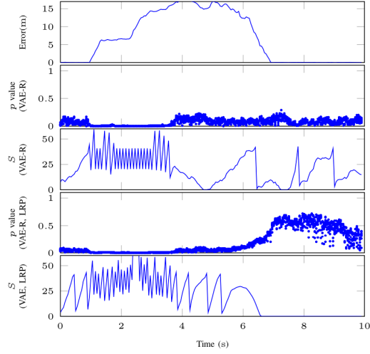
Fig. 6. Episode with dataset shift (target shift).
