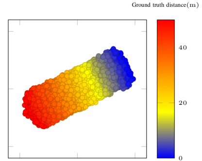
Fig. 3. 2-dimensional latent representations estimated by VAE for regression.
