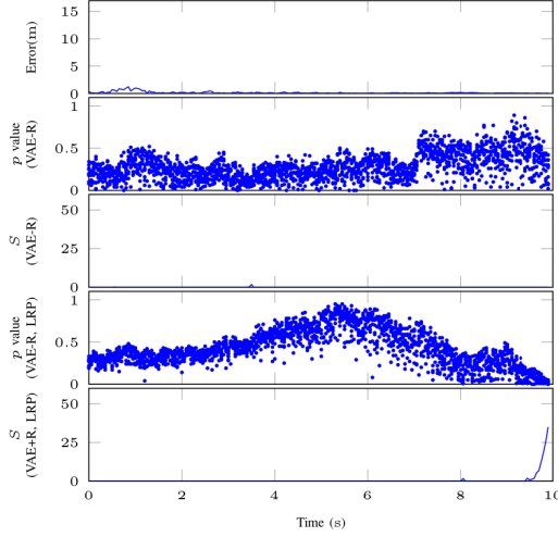
Fig. 4. Episode with in-distribution inputs.
