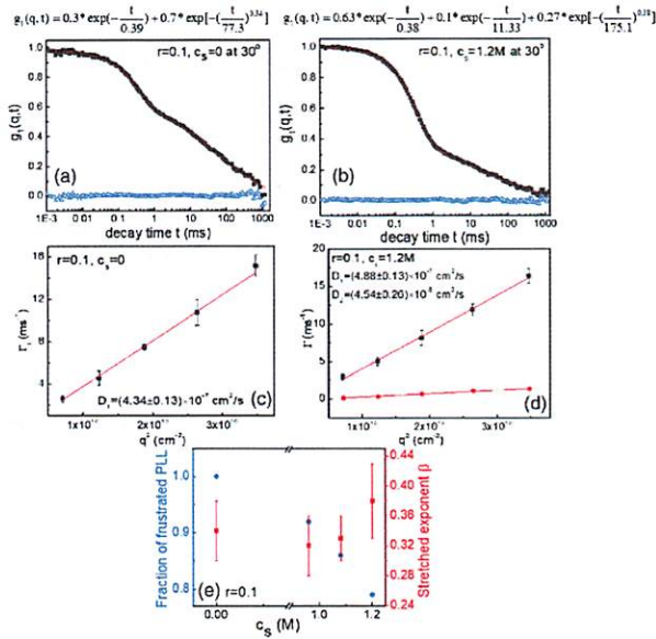
FIG. 3. (a),(b) Normalized field correlation function g_1(t) at scattering angle 30^\circ for r = 0.1 and c_s = 0 and 1.2M (red lines are the best fits and blue triangles are residuals). (c),(d) Corresponding q^2 dependence of relaxation rates \Gamma . (e) Stretched exponent \beta and the fraction of frustrated PLL for r = 0.1 ( c_p = 1 mg/mL) at different salt concentrations.
