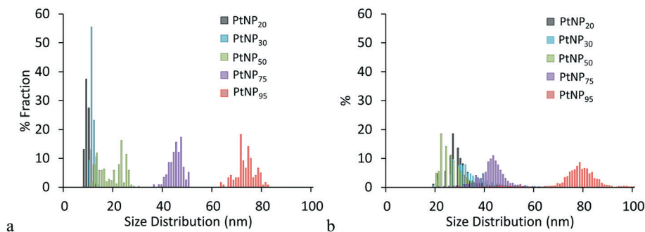
Fig. 1 Number particle size distribution of polyvinylpyrrolidone-coated platinum nanoparticles of five different nominal sizes ranging from 20 to 95 nm (denoted as PtNP 20 –PtNP 95 ) measured by (a) transmission electron microscope (TEM), and (b) single particle-inductively coupled plasma-mass spectrometer (sp-ICP-MS). Size detection limit of PtNPs in sp-ICP-MS is 18 nm.
