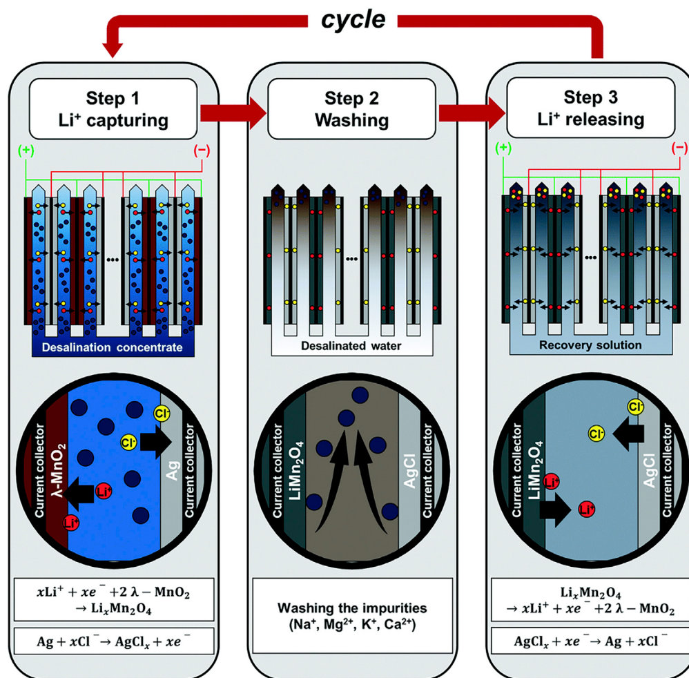
Figure 9. Schematic illustration of a three-step process for continuous recovery of lithium using \lambda - \text{MnO}_2/\text{Ag} electrode in a pilot-scale system
