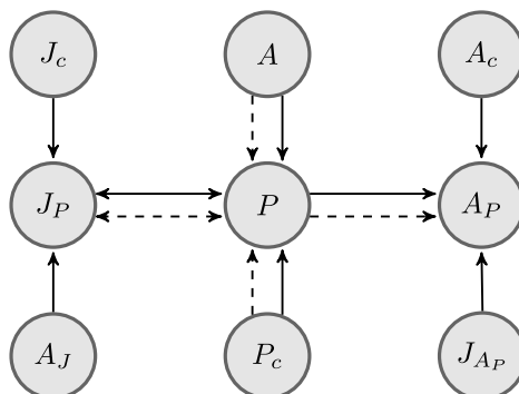
Fig. 2. Comparison of the flow of importance of the BDR three-class model and our three-class model. Solid lines show the flow of importance in the BDR three-class model and dashed lines show the flow of importance in our three-class model. Here A denotes the author or set of co-authors of paper P , J_p denotes the journal where paper P is published, P_c denotes the set of papers that cite paper P , A_p stands for one of the authors of paper P , A_c stands for set of co-authors of author A_p , J_{A_p} denotes the set of journals where author A_p 's papers are published, J_c denotes the set of journals that contain papers that cite papers published in journal J_p , and A_j denotes the set of authors who publish their papers in journal J_p .
