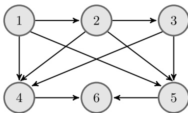
Fig. 6. Directed network of Example 4.5.
