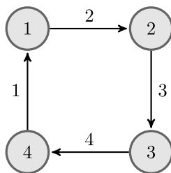
Fig. 5. Directed network of Example 4.3.
