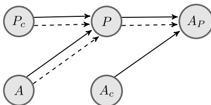
Fig. 1. Comparison of the flow of importance of the BDR two-class model and the two-class model of Section 5. Solid lines show the flow of importance in the BDR two-class model and dashed lines show the flow of importance in the two-class model of Section 5. Here A stands for the author or set of co-authors of paper P , P_c stands for the set of papers that cite paper P , A_p stands for one of the authors of paper P , and A_c stands for the co-authors of author A_p .
