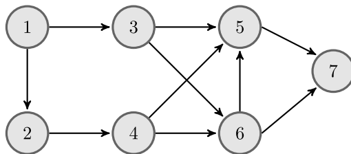
Fig. 4. Directed network of Example 4.2.
