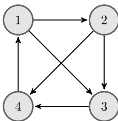
Fig. 7. Directed network of Example 4.6.
