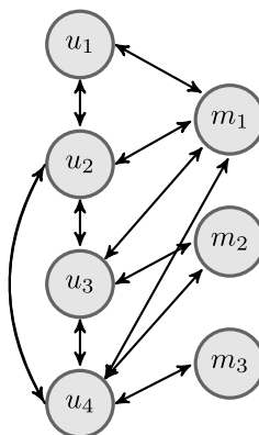
Fig. 8. Directed network of Example 5.1.
