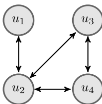
Fig. 3. Undirected network of Example 4.1.
