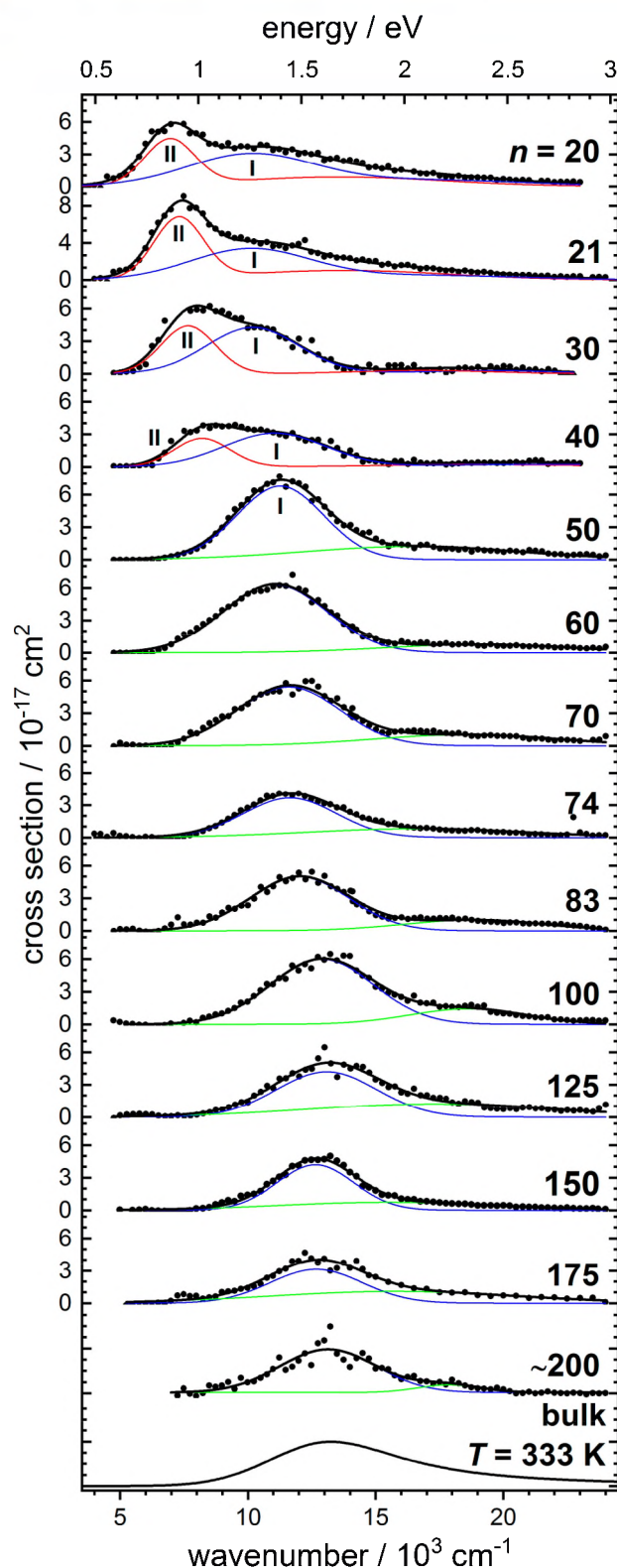
Figure 1. Optical absorption spectra of (\text{H}_2\text{O})_n^- in the cluster size region of n = 20\text{--}200 at T = 80\text{ K} . The bulk spectrum of the hydrated electron in water at 333\text{ K} ( 60\text{ }^\circ\text{C} ) from ref 23 is shown for comparison.
