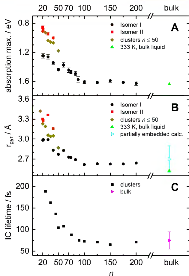
Figure 2. (A) Optical absorption maxima of Isomers I and II (this work) compared with maxima for clusters n \leq 50 from ref 7 and e_{\text{hyd}} in bulk liquid at 333\text{ K} from ref 23. (B) Electron gyration radius for the systems in panel (A) compared with calculations of the partially embedded isomer from ref 27. (C) Internal conversion (IC) lifetime of the hydrated electron in (\text{H}_2\text{O})_n^- clusters from ref 12 and in bulk from ref 25 shown for comparison.
